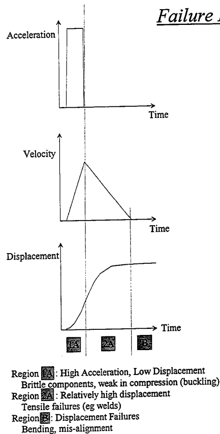
Figure 8. Time-history response regions relating to shock induced damage of equipment.
