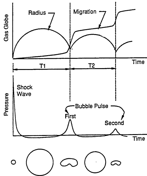
Figure 1. Bubble migration behaviour versus bubble expansion [2].
