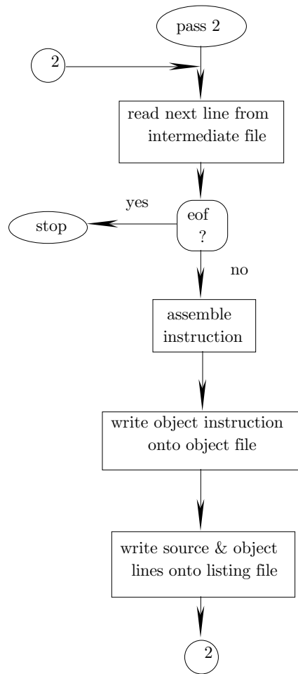
Figure 1–2. The Operations of the Two-Pass Assmbler (part 2).
