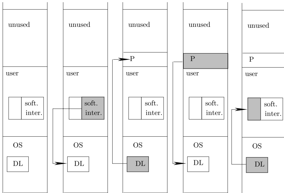
Figure 7-6. Dynamic Linking.
