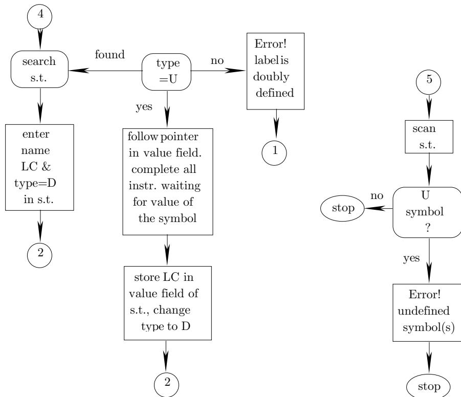
Figure 1–3. The Operations of the One-Pass Assmbler (part 2).
