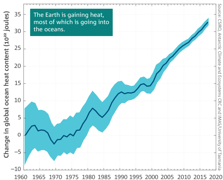
Estimated change in ocean heat content over the full ocean depth, from 1960 to 2017. Shading provides an indication of the confidence range of the estimate. Note that data contributing to the early part of the record are sparse and trends estimated over this period are small compared to the error bars, hence considered unreliable.
