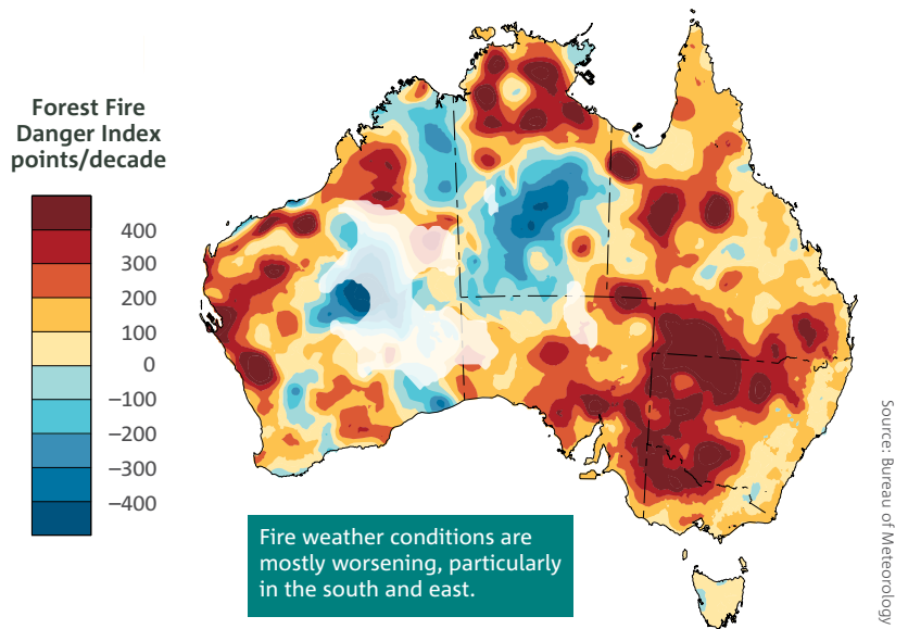
Trends from 1978 to 2017 in the annual (July to June) sum of the daily Forest Fire Danger Index—an indicator of the severity of fire weather conditions. Positive trends, shown in the yellow to red colours, are indicative of an increasing length and intensity of the fire weather season. A trend of 300 FFDI points per decade is equivalent to an average trend of 30 FFDI points per year. Areas where there are sparse data coverage such as central parts of Western Australia are faded.
