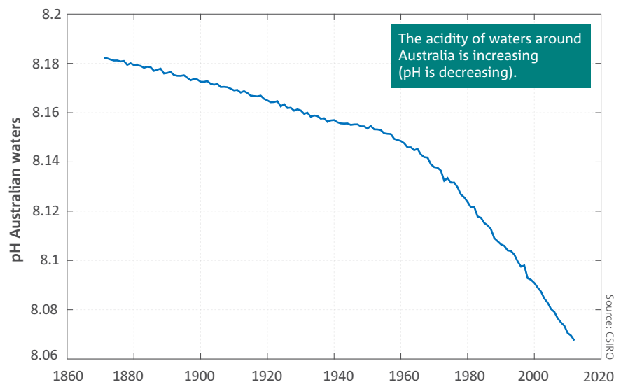
The pH of surface waters around Australia, top: change between 1880–1889 and 2003–2012, bottom: the average pH of water surrounding Australia. Calculations are based on present-day data on the carbonate chemistry of surface seawater around Australia from the Integrated Marine Observing System and other programs, and extrapolation of atmospheric carbon dioxide concentration changes since the 1880s. Source: CSIRO, Lenton et al. (2016).
