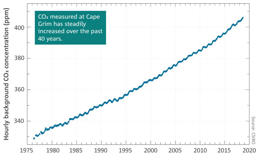
Background hourly clean-air CO 2 as measured at the Cape Grim Baseline Air Pollution Station through to September 2018. The blue hourly data represent thousands of individual measurements. To obtain clean air measurements, the data are filtered to only include times when weather systems come across the Southern Ocean, and thus the air is not influenced by local sources of pollution.
