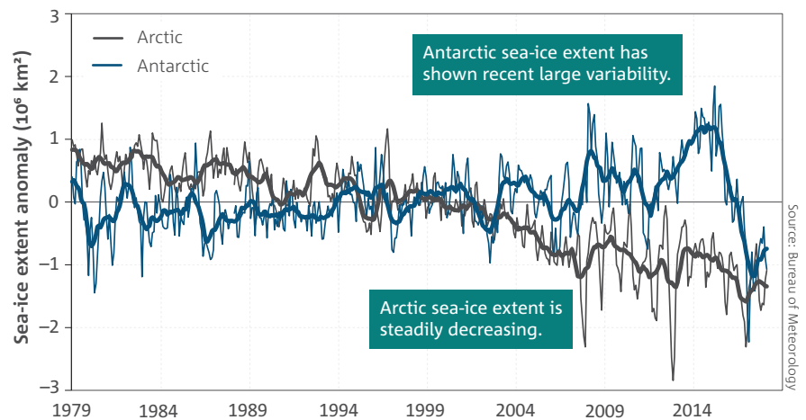
Antarctic and Arctic sea-ice extent (shown as the net anomaly from the 1981–2010 average) for the period January 1979 to May 2018 (10 6 km 2 ). Thin lines are monthly averages and indicate the variability at shorter time-scales, and thick lines are eleven-month running averages.
