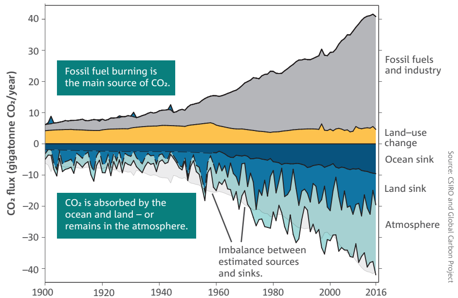
The CO 2 fluxes in the global carbon budget over the period 1900–2016.
