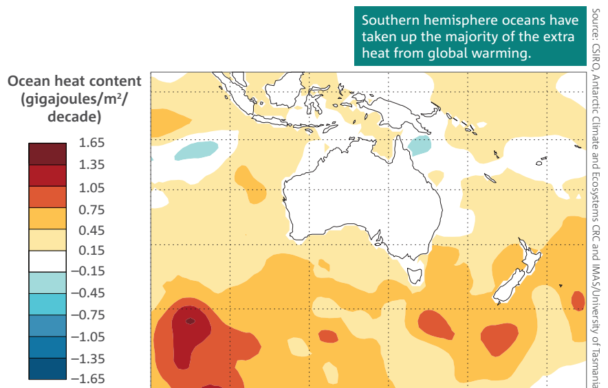
Estimated linear trend in ocean heat content between 1970 and 2017 in the top 700 m of the ocean, showing the highest uptake of heat in regions where ocean currents move heat to the deep ocean such as the Southern Ocean south of Australia.
