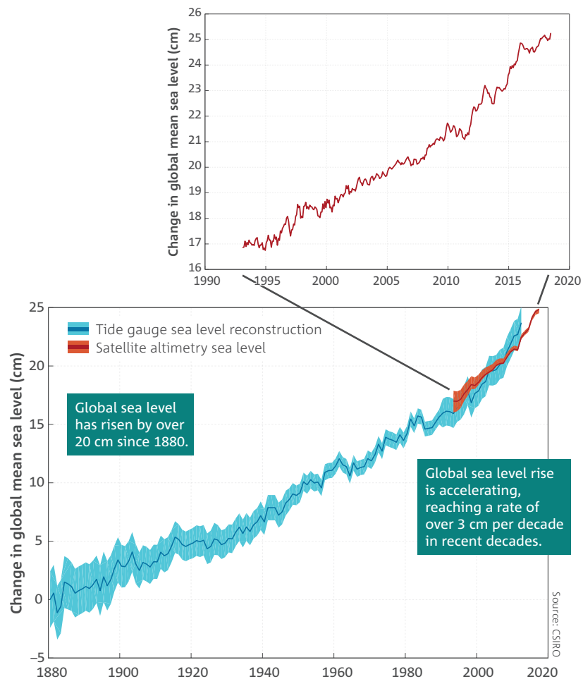
High-quality global sea level measurements showing annual sea level change from 1880 in tide gauge data (1880–2014 blue line, light blue shading indicates confidence range), and annual sea level change in satellite altimetry (1993–2017, red line). The pull out figure shows monthly sea level change from 1880 in satellite altimetry from 1993 to July 2018 (updated from Church and White 2011). https://research.csiro.au/slrwavescoast/sea-level/ .
