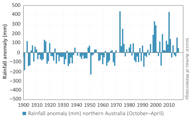
Anomalies of October to April rainfall for northern Australia (north of 26° S inclusive). Anomalies are calculated with respect to the 1961 to 1990 average.
