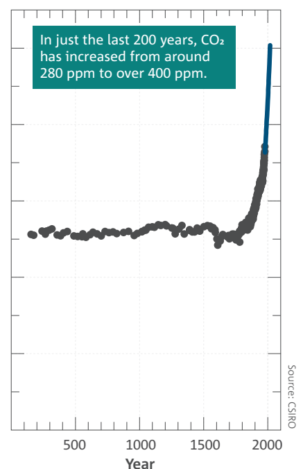
Atmospheric CO 2 concentrations from 800,000 years ago to around year 0, and for the last 2017 years, from measurements of air in Antarctic ice cores and at Cape Grim.
