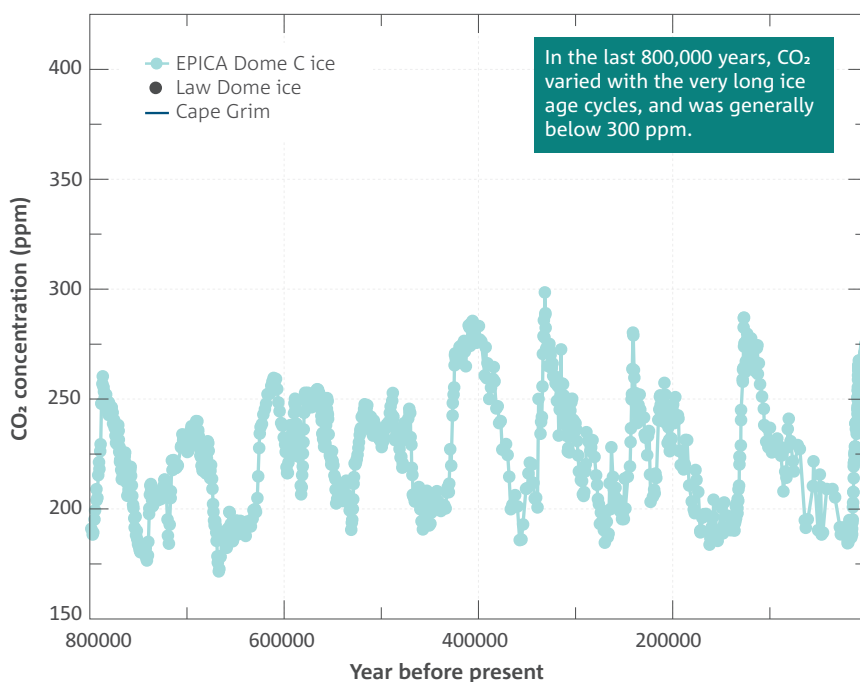
Atmospheric CO 2 concentrations from 800,000 years ago to around year 0, and for the last 2017 years, from measurements of air in Antarctic ice cores and at Cape Grim.
