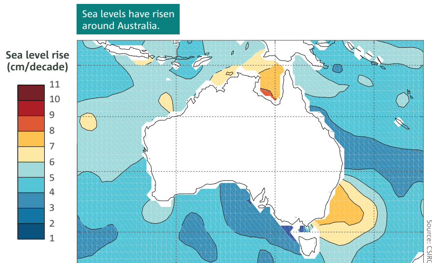
The rate of sea level rise around Australia by satellite observations from 1993 to 2017. Source: CSIRO, update from White et al. (2014).
