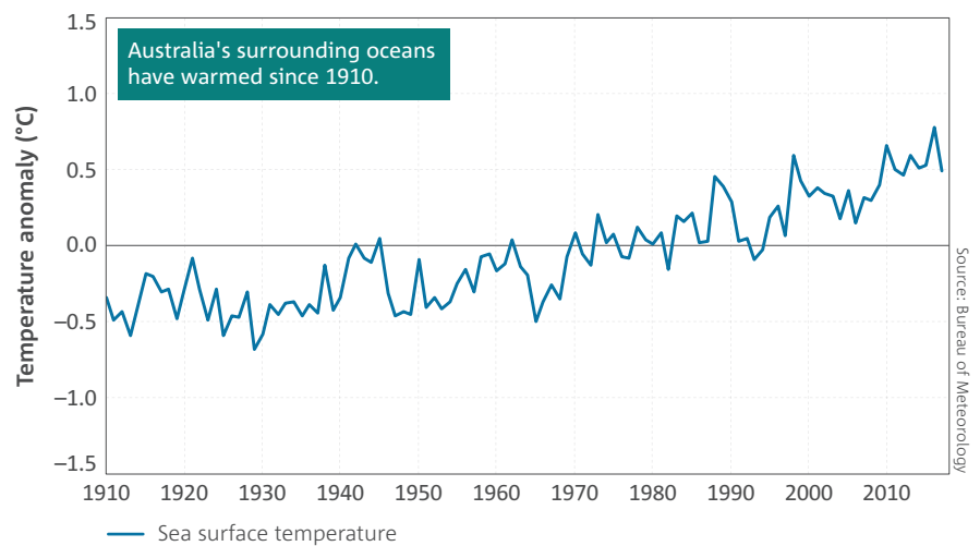
Anomalies in annual sea surface temperature in the Australian region. Anomalies are the departures from the 1961–1990 standard averaging period. Sea surface temperatures are for the Australian region (4–46° S and 94–174° E).
