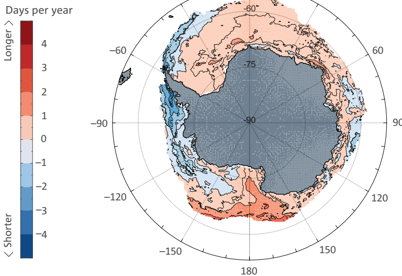
Trend in sea-ice season duration (1979–2017)
