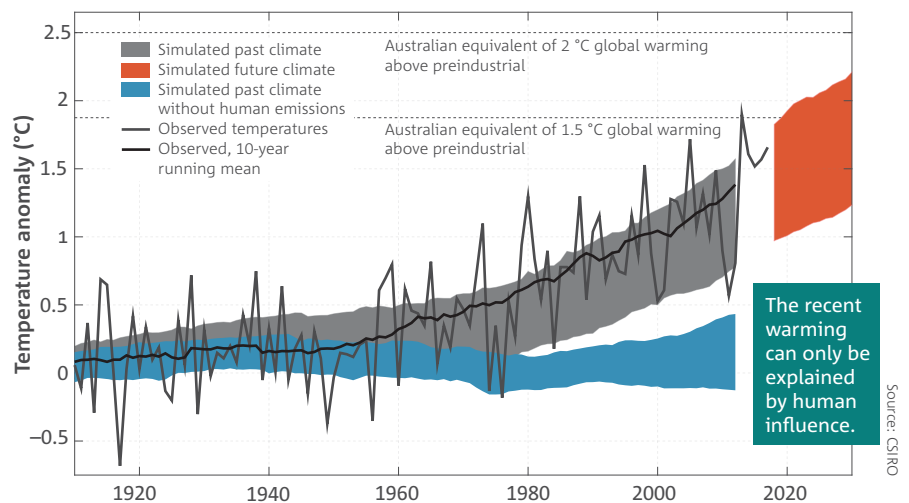
Australia's average annual temperature relative to the 1861–1900 period. The grey line represents Australian temperature observations since 1910, with the black line the ten-year running mean. The shaded bands are the 10–90% range of the 20-year running mean temperatures simulated from the latest generation of Global Climate Models. The grey band shows simulations that include observed conditions of greenhouse gases, aerosols, solar input and volcanoes; the blue band shows simulations of observed conditions but not including human emissions of greenhouse gases or aerosols; the red band shows simulations projecting forward into the future (all emissions scenarios are included). Warming over Australia is expected to be slightly higher than the global average. The dotted lines represent the Australian equivalent of the global warming thresholds of 1.5 °C and 2 °C above preindustrial levels, which are used to inform possible risks and responses for coming decades.
