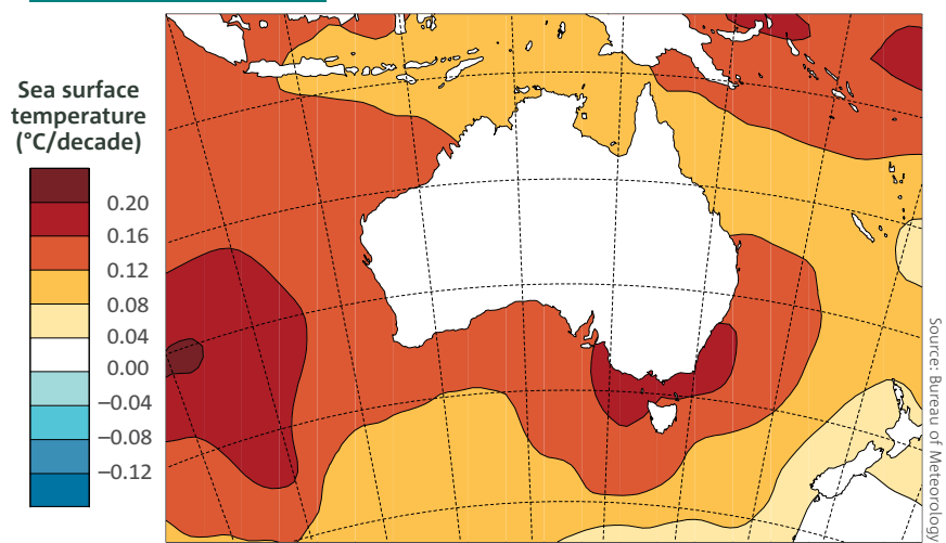
Trends in sea surface temperatures in the Australian region from 1950 to 2017 (data source: ERSST v5, www.esrl.noaa.gov/psd/ ).
