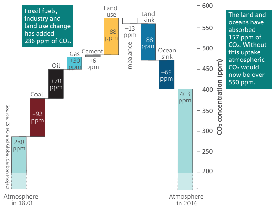
The cumulative contributions to the global carbon budget from 1870 to 2016. Visualising the difference between the year 1870 and 2016, the cumulative drivers of increase (sources) on one side, and the drivers of decrease (sinks) on the other side explains the increase in atmospheric concentration of CO 2 . The small remaining carbon imbalance represents the gap in the current understanding and estimates of sources and sinks.
