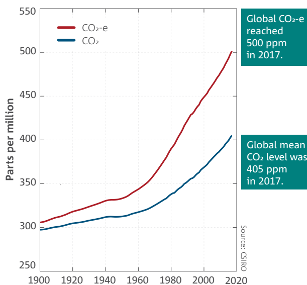
Left: Radiative forcing relative to 1750 due to the long-lived greenhouse gases carbon dioxide, methane, nitrous oxide and the synthetic greenhouse gases, expressed as watts per metre squared. Right: Global mean CO 2 concentration and global mean greenhouse gas concentrations expressed as equivalent CO 2 (ppm: parts per million). Data in both panels are from in situ monitoring by CSIRO and the Bureau of Meteorology (commencing Cape Grim, Tasmania, 1976) and the Advanced Global Atmospheric Gases Experiment (global, including Cape Grim, commencing 1978) and from measurements of flask air samples (global, including Cape Grim, commencing 1992), the Cape Grim Air Archive (1978–2017) at the CSIRO GASLAB (Aspendale, Melbourne) laboratory, and air from Antarctic firn (compact snow) and ice cores measured at CSIRO GASLAB and ICELAB (Aspendale, Melbourne). Equivalent CO 2 is calculated from the atmospheric concentrations of carbon dioxide, methane, nitrous oxide and the suite of synthetic greenhouse gases.
