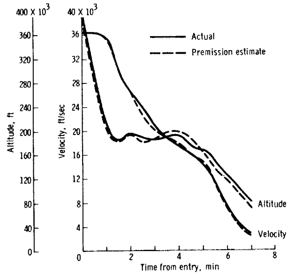
Figure 13. - Apollo 10 velocity and altitude time histories.
