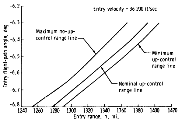
Figure 10. - Up-control breakpoint.
