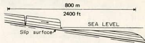
Figure 2.14. Section view of translational slide at Point Fermin, near Los Angeles, California (see also Figure 2.15) (2.107, 2.182).
