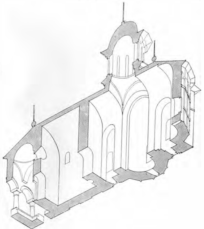
Fig. 34. — Perspective
