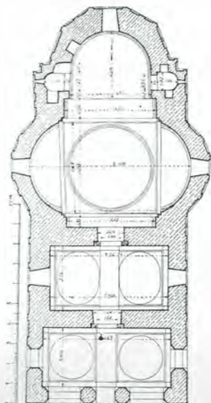
Fig. 196. — Plan
