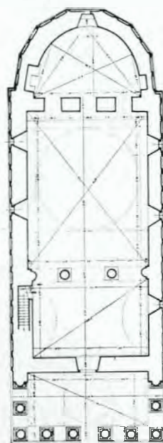
Fig. 286. — Plan
