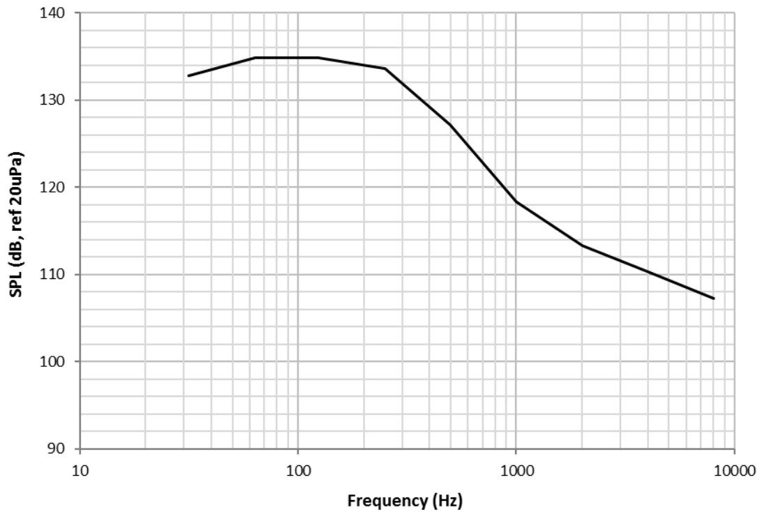
Figure 4-8: Falcon Heavy maximum predicted acoustic environment (P95/50), 60% fill-factor, 140.3 dB OASPL (full octave)
