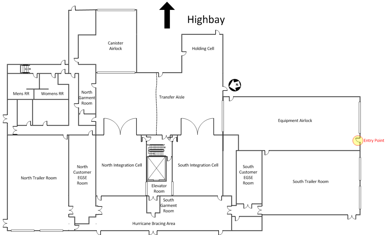
Figure 8-3: CCAFS PPF East Bay floor plan
