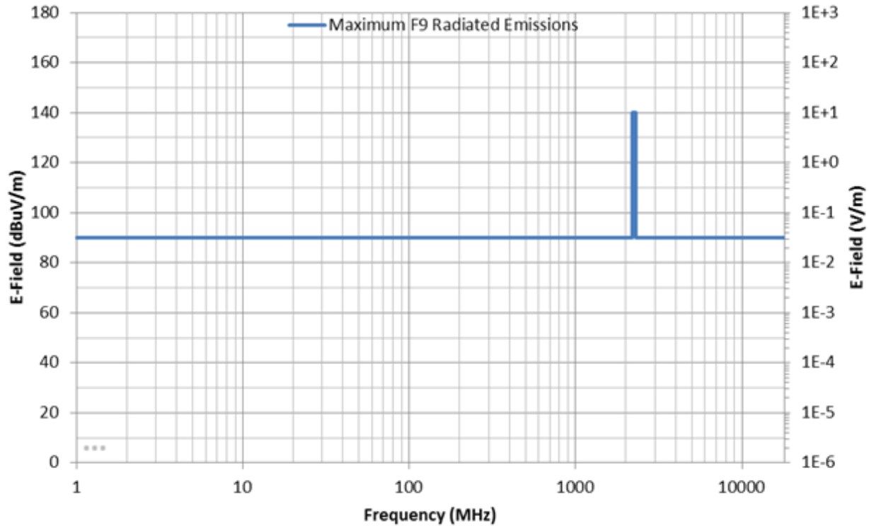
Figure 4-11: Falcon 9 worst-case radiated environment
