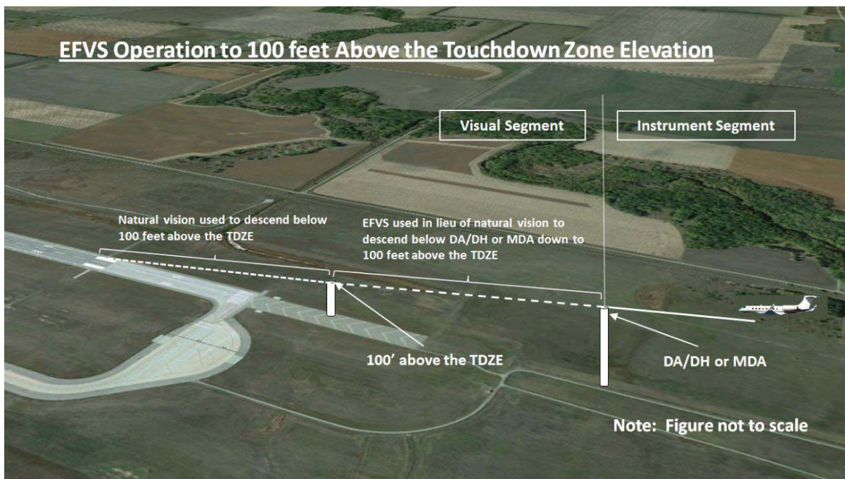
FIG 5-4-34 EFVS Operation to 100 ft Above the TDZE [Photo provided by Google Earth]
