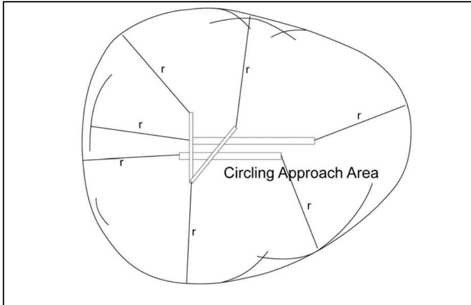
FIG 5-4-28 Final Approach Obstacle Clearance
