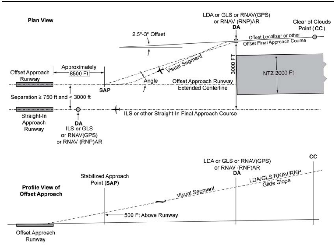
FIG 5-4-24 SOIA Approach Geometry
