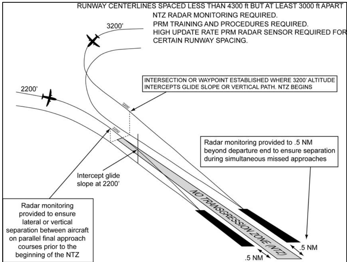
FIG 5-4-23 PRM Approaches Simultaneous Close Parallel
