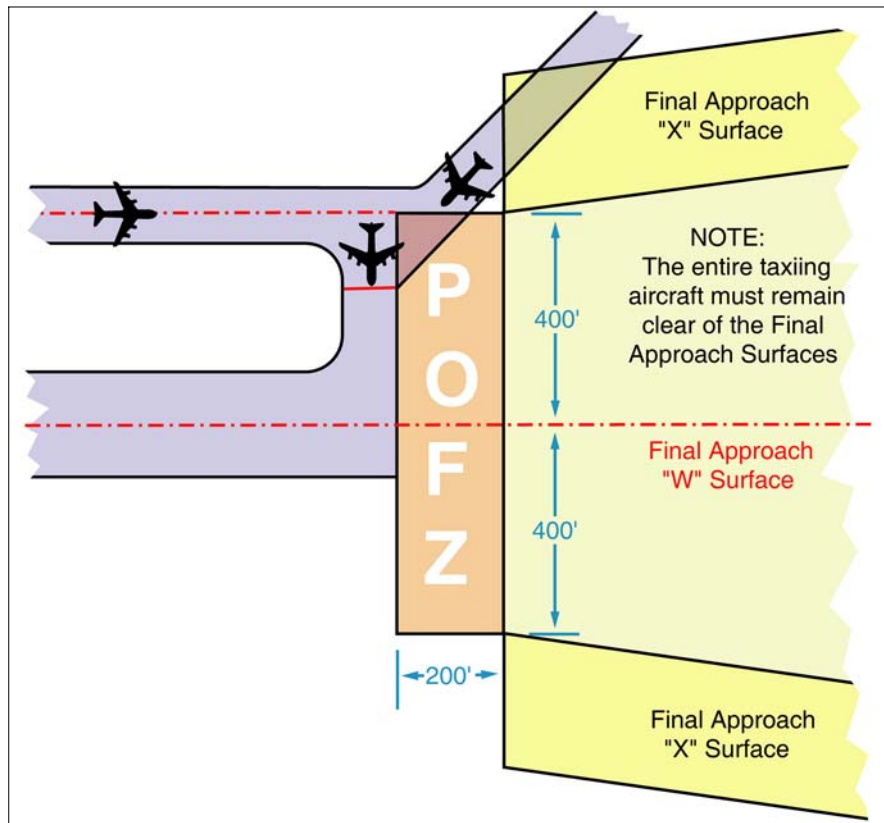
FIG 5-4-30 Precision Obstacle Free Zone (POFZ)
