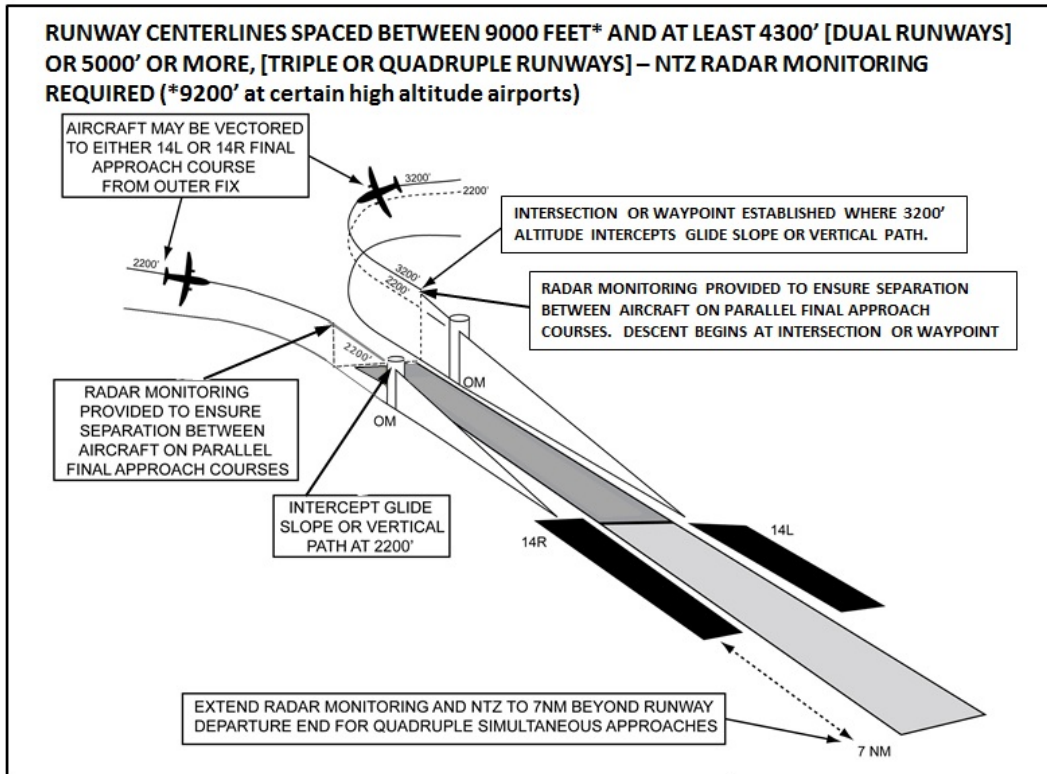
FIG 5-4-22 Simultaneous (Parallel) Independent ILS/RNAV/GLS Approaches
