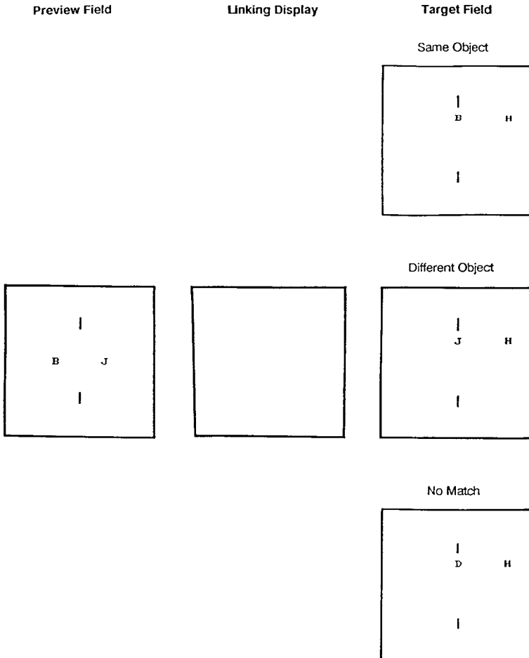
FIG. 2. Examples of displays used in Experiment 3 with apparent motion.
