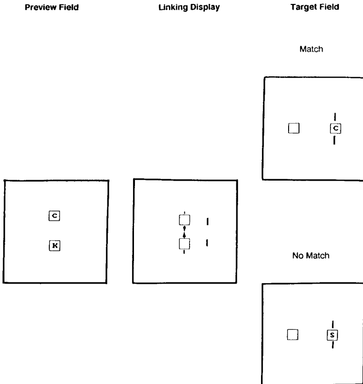
FIG. 5. Examples of displays used in Experiment 6(b).
