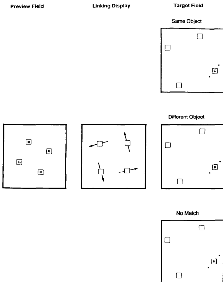
FIG. 4. Examples of displays used in Experiment 5.
