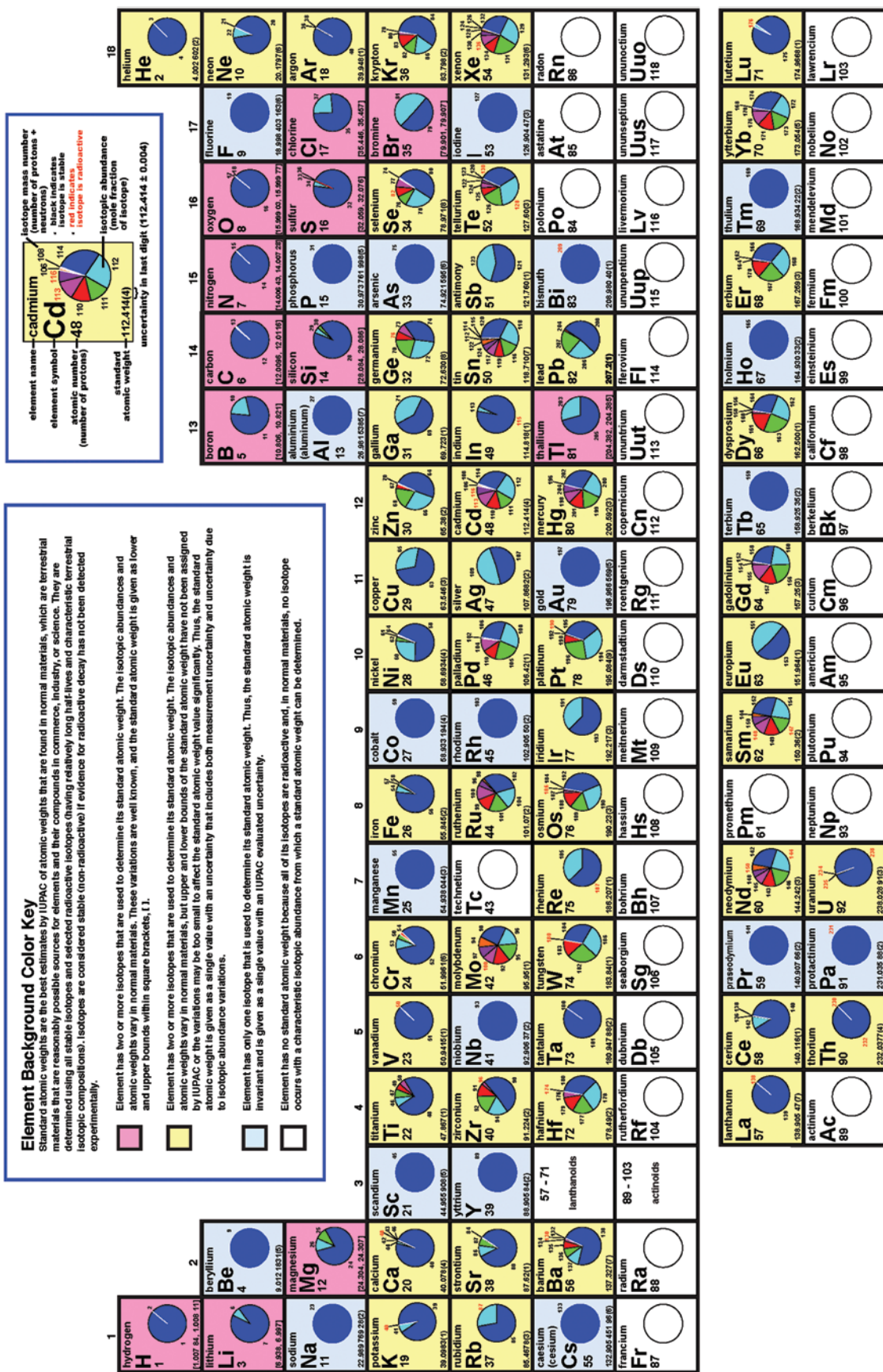
International Union of Pure and Applied Chemistry (IUPAC) Project 2007-038-3-200, "Development of an isotopic periodic table for the educational community" October 1, 2013 www.iaaw.org
