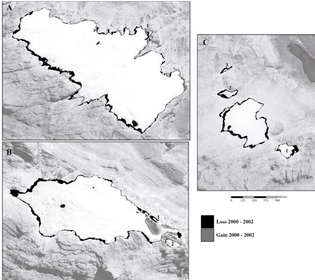
Figures 3A, B, and C represent the digitizing results for the E. Northwall Firn, the Carstensz Glacier, and the W. Northwall Firn, respectively.
