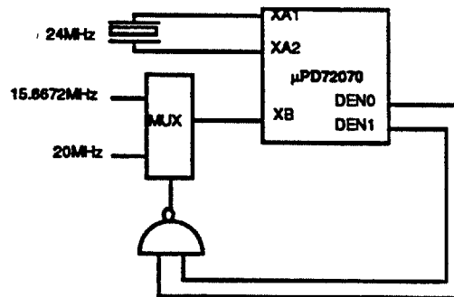
Recommended Circuit #2
