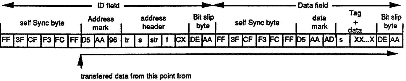
Fig. 4.18.3 Transferred Data for Dump After Data Address Mark
