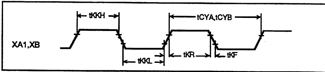
Fig.1 External Clock
