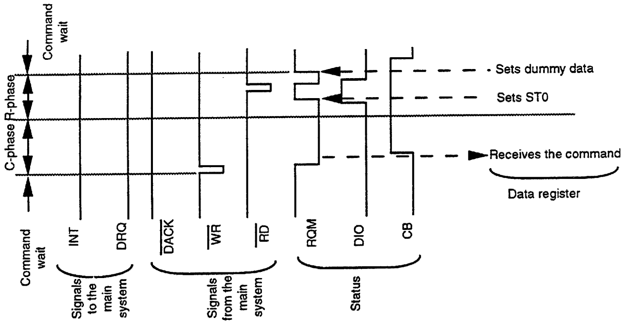
Fig.5.1-10 INVALID command
