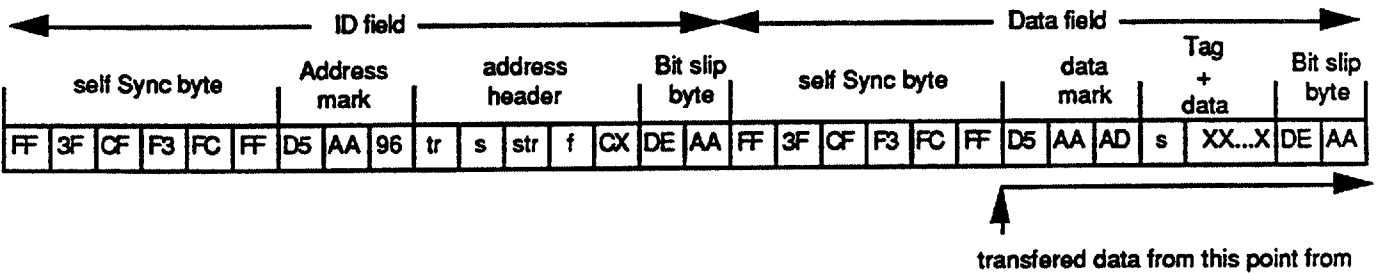
Fig. 4.18.2 Transferred Data for Dump After Specified ID Address Mark
