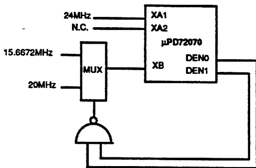
Recommended Circuit #1
