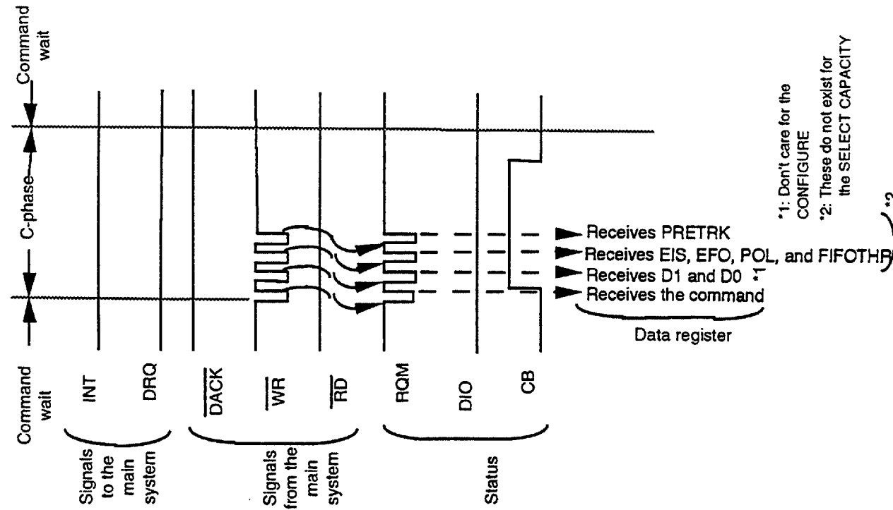
Fig.5.1-8 CONFIGURE and SELECT CAPACITY commands
