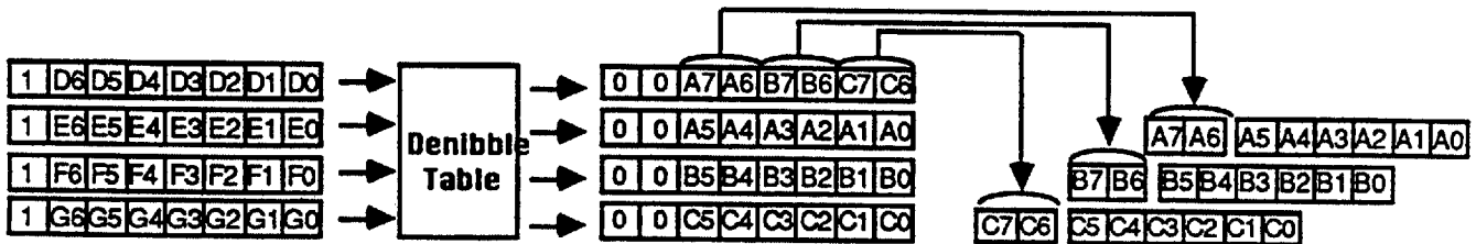
Fig. 1.3.5 Denibbling process for Sector Data
