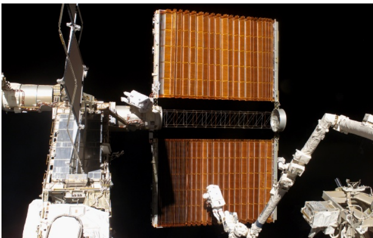
S116-E-06854 - FD10: EVA 4 Curbeam & Fuglesang (out of frame), working in tandem, used specially-prepared tape insulated tools to guide the P6 overhead SAW neatly inside its blanket box.
