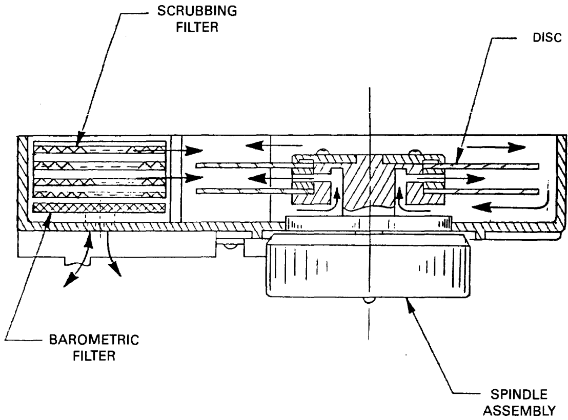
FIGURE 1B AIR FILTRATION SYSTEM
