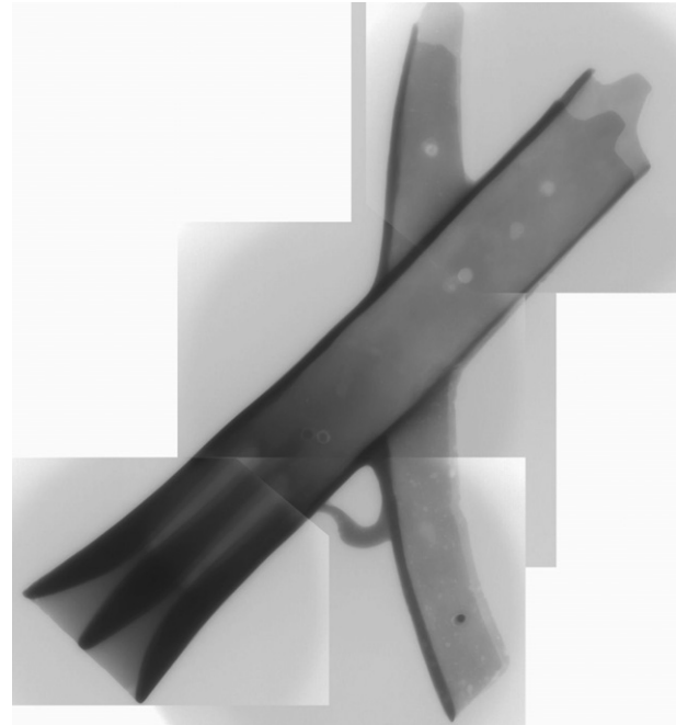
Figure 11. Composite radiograph of the ram. This is a positive image so that thicker metal is darker. (Crown copyright)
