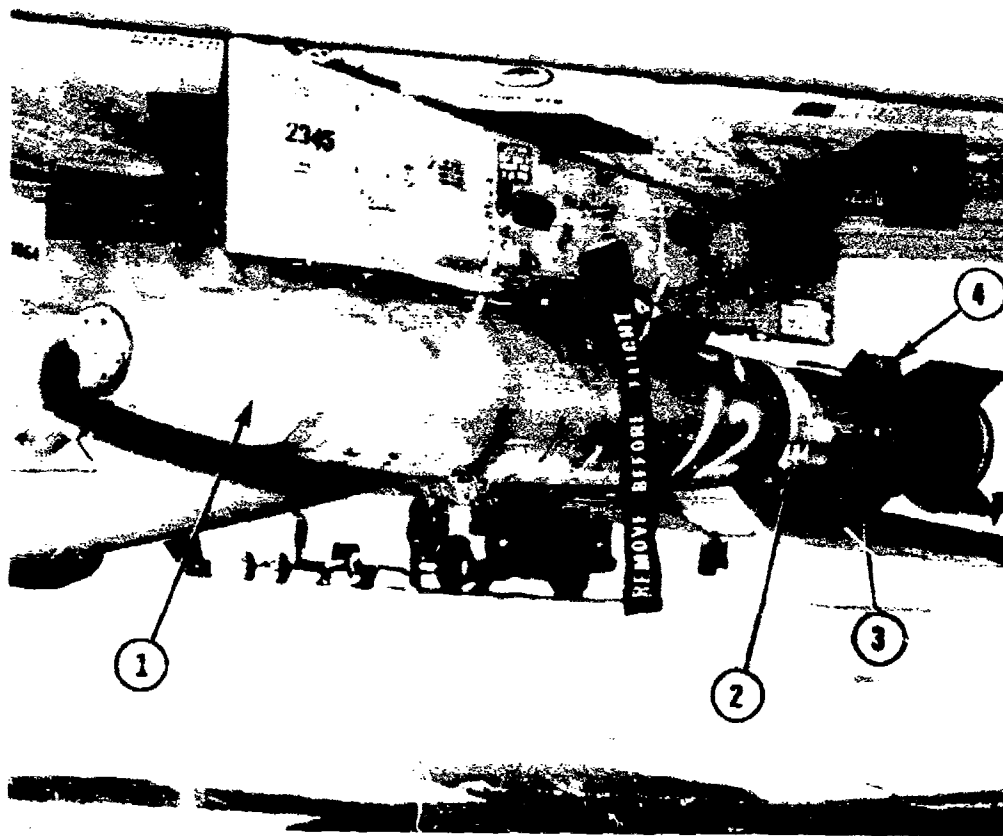
Figure 1. MK 82 bomb with ballute retarder system on an F-100 outboard pylon: (1) MK 82 bomb, (2) retaining clamp, (3) finned canister, and (4) mechanical timer
