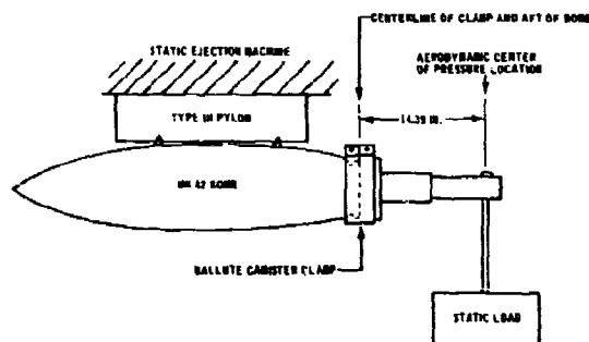
Figure 6. Static load test arrangement
