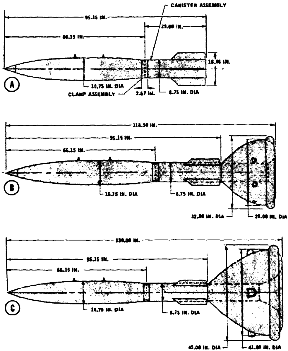
Figure 3. Physical comparison of the ballute retarder systems: (A) low drag, (B) 29-inch high drag, and (C) 41-inch high drag
