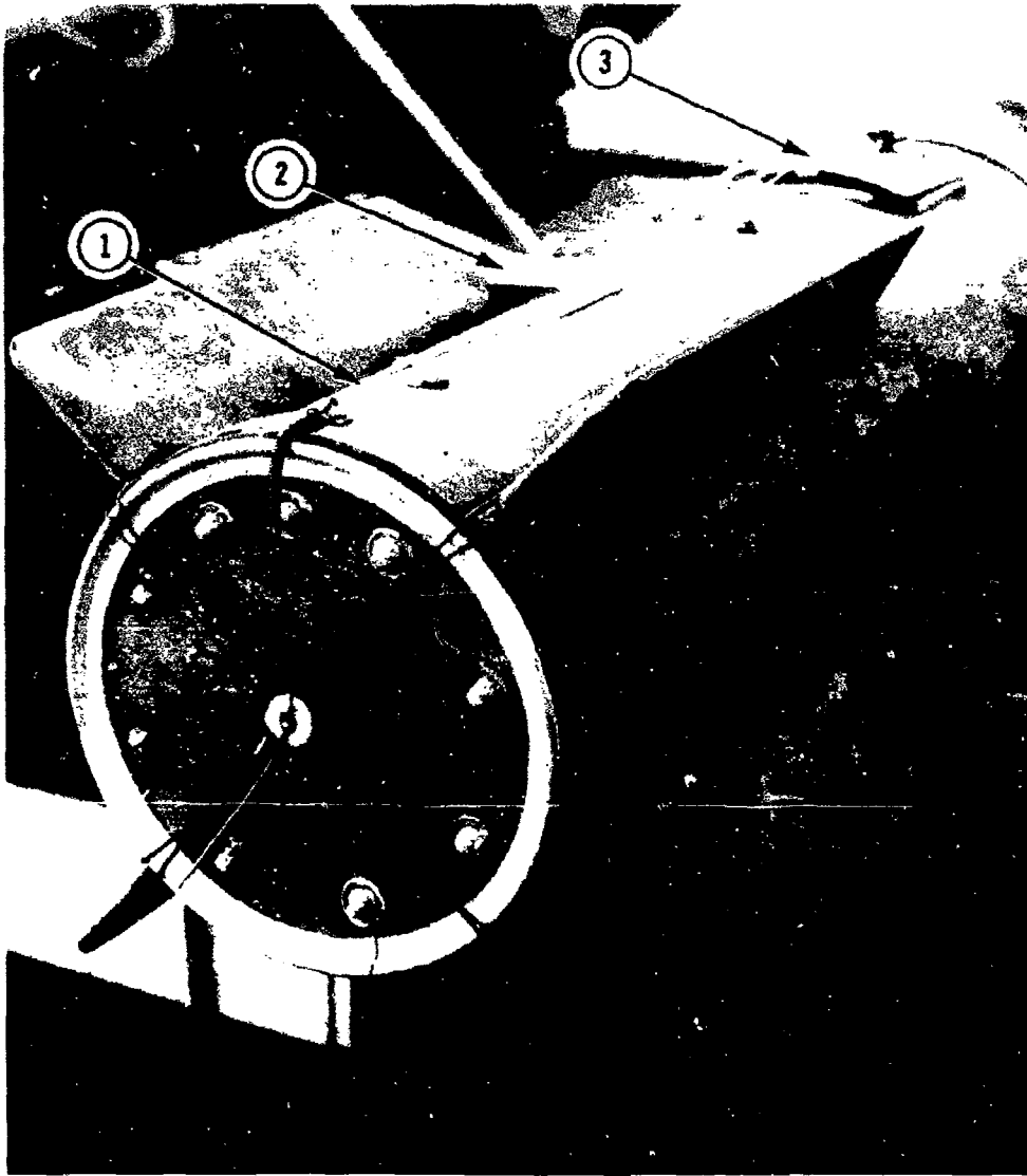
Figure 5. Type II release mechanism (arrows) and (1) lanyard, (2) mechanical timer mount, and (3) popup air scoop
