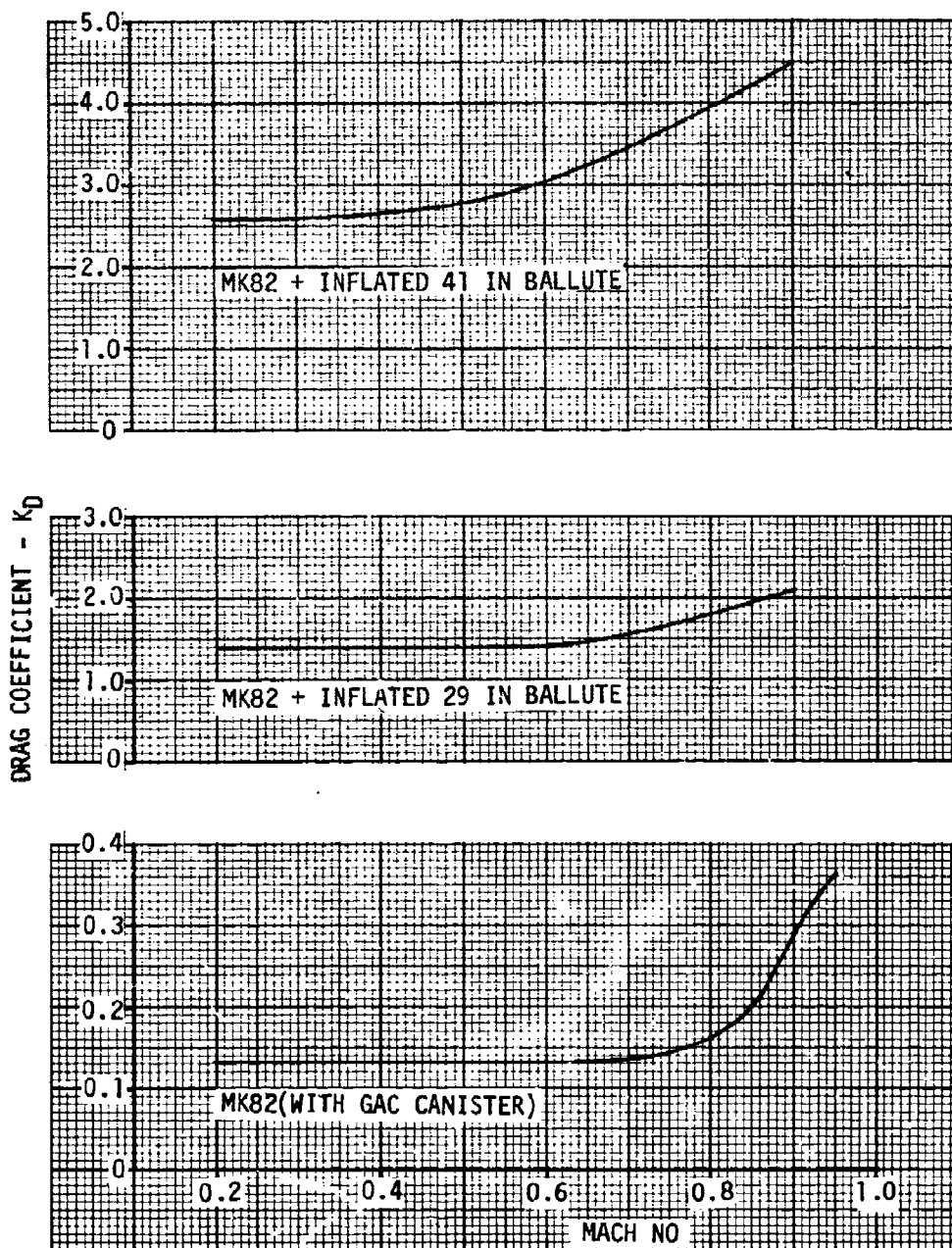
Figure II-1. Drag coefficients of MK 82 bomb with GAC ballutes and canister
