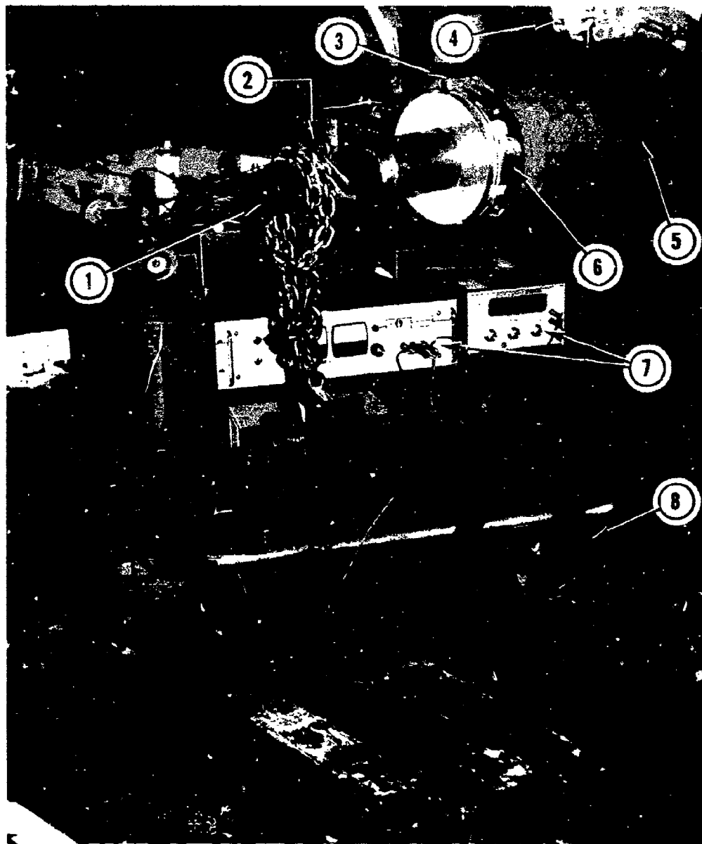
Figure 7. Static load test setup and strain gage locations: (1) adapter, (2) aerodynamic center of pressure, (3) redesigned retaining clamp, (4) pylon, (5) MK 82 bomb, (6) strain gage, (7) instrumentation, and (8) weights
