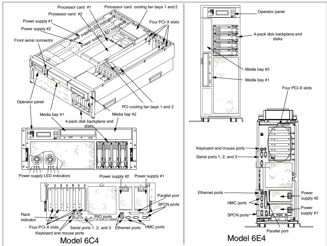
Figure 1-1 Views of Models 6C4 and 6E4
