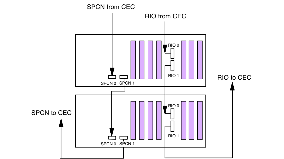
Figure 2-7 Remote I/O and SPCN cabling
