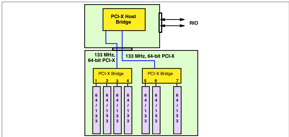
Figure 2-6 Conceptual diagram of the I/O drawer
