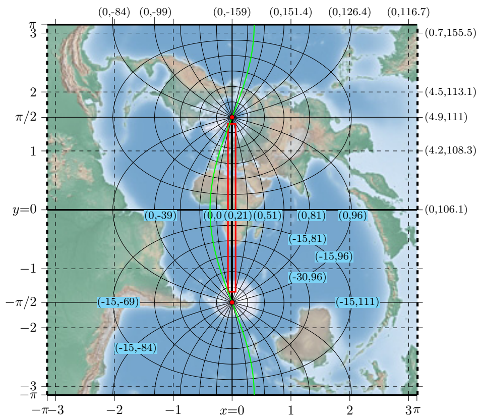
Figure 3.4: Transverse Mercator centred on 21E
