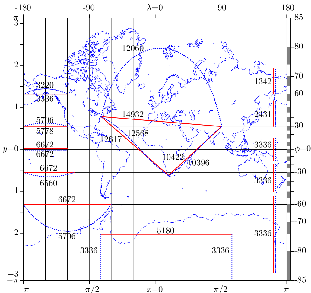
Figure 2.16: Rhumb lines (red) and shorter great circles (blue dash)
