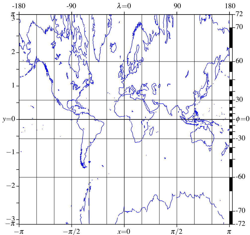
Figure 2.11: Central cylindrical projection truncated at 72° (R=1)
