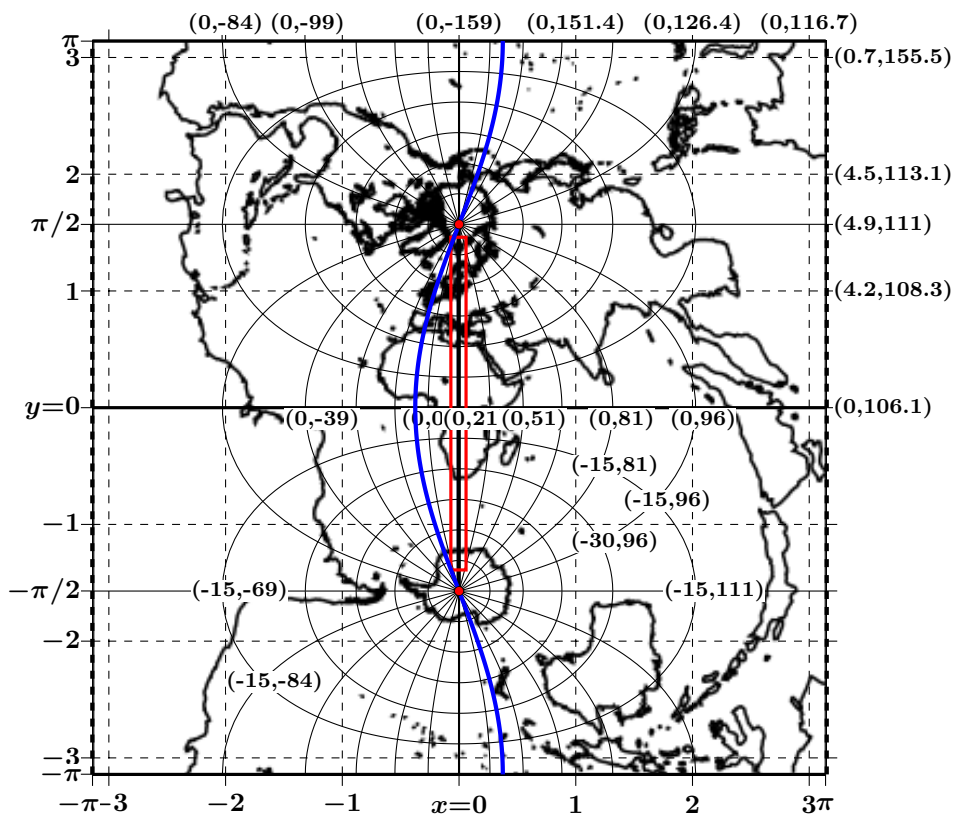
Figure 3.7 : Transverse Mercator centred on Greenwich (top) and 21E (bottom)
