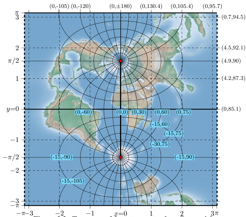
Figure 3.3 : Transverse Mercator centred on Greenwich
