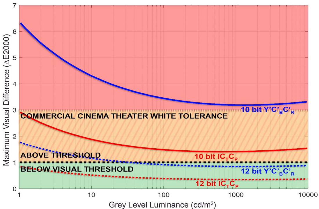
Figure 10: Baseband quantization comparison at 10 and 12 bits
