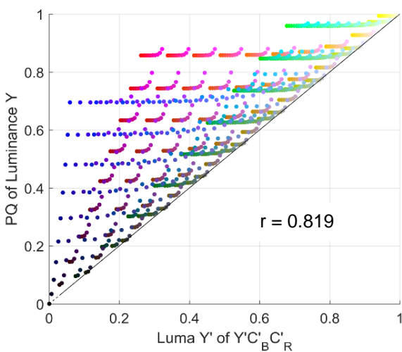
Figure 3: PQ based BT.2020 NCL Y'C'_B'C'_R luminance analysis
