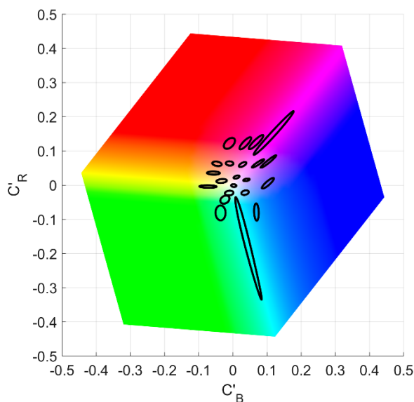
Figure 7: PQ based BT.2020 NCL Y'C'_B C'_R JND analysis
