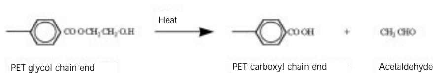
Figure 3. Acetaldehyde formation
