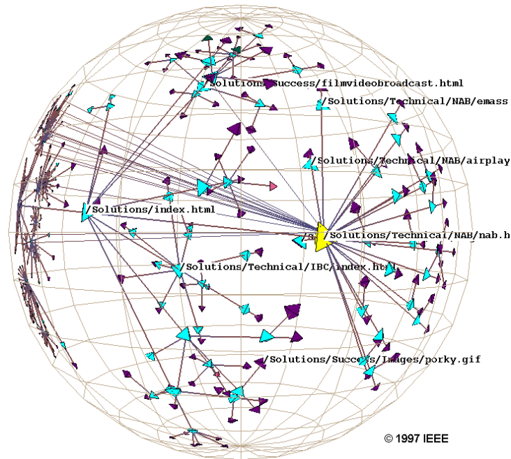
Fig. 12. Hyperbolic Tree
