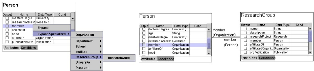
Fig. 11. Selecting a property (left) and the expanded node (right)
