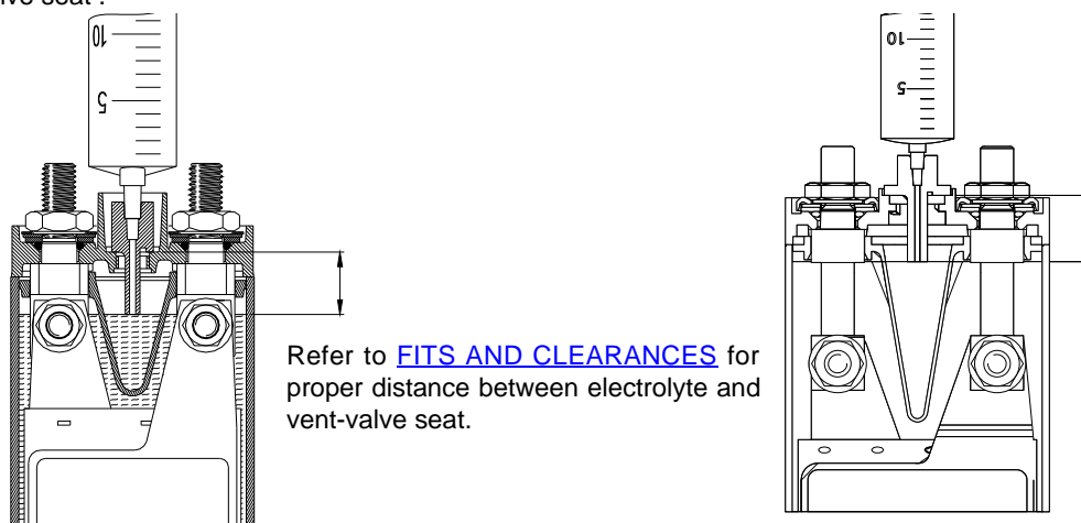
Position of Syringe in Cell Vent Seat Figure 2
