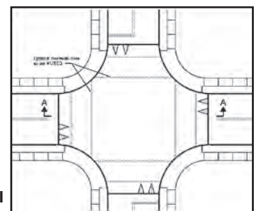
Image source: Delaware DOT Traffic Calming Manual
