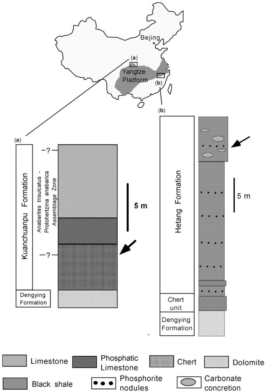
Fig. 1. Sample location areas on the Yangtze Plate, China and stratigraphic columns. Arrows point to radiolarian-bearing horizons. (a) Stratigraphic column of the Kuanchuanpu Formation at Shizonggou, near Kuanchuanpu, Ningqian County (Shaanxi Province). (b) Stratigraphic column of the Hetang Formation at Xintangwu, Jianshan County, W. Zhejiang Province.
