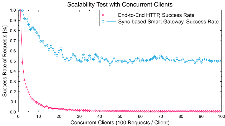
Figure 3.10: Comparing the scalability in terms of concurrent requests for the end-to-end HTTP and the syn-based Smart Gateway version. Each client runs a 100 requests and the clients are concurrently started. The Smart Gateway version scales much better.
