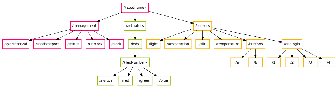
Figure 3.4: Resources of the Sun SPOT RESTful API as offered by the DeviceDriver through the Smart Gateway.
