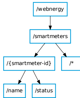
Figure 3.16: RESTful Web API of the Webnergy framework. The functionality of these resources is listed in Table 3.1.
