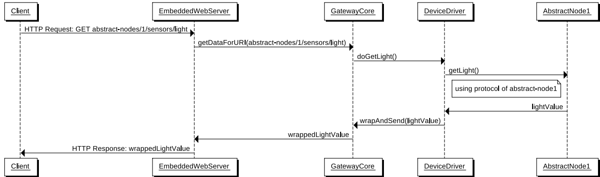
Figure 2.7: Simplified sequence diagram of the interaction between a client and a smart thing through a Smart Gateway. The Smart Gateway framework delegates the invocation to the corresponding Device Driver and takes care of converting the results into the appropriate format (e.g., JSON) and wrapping them into an HTTP packet returned to the client.
