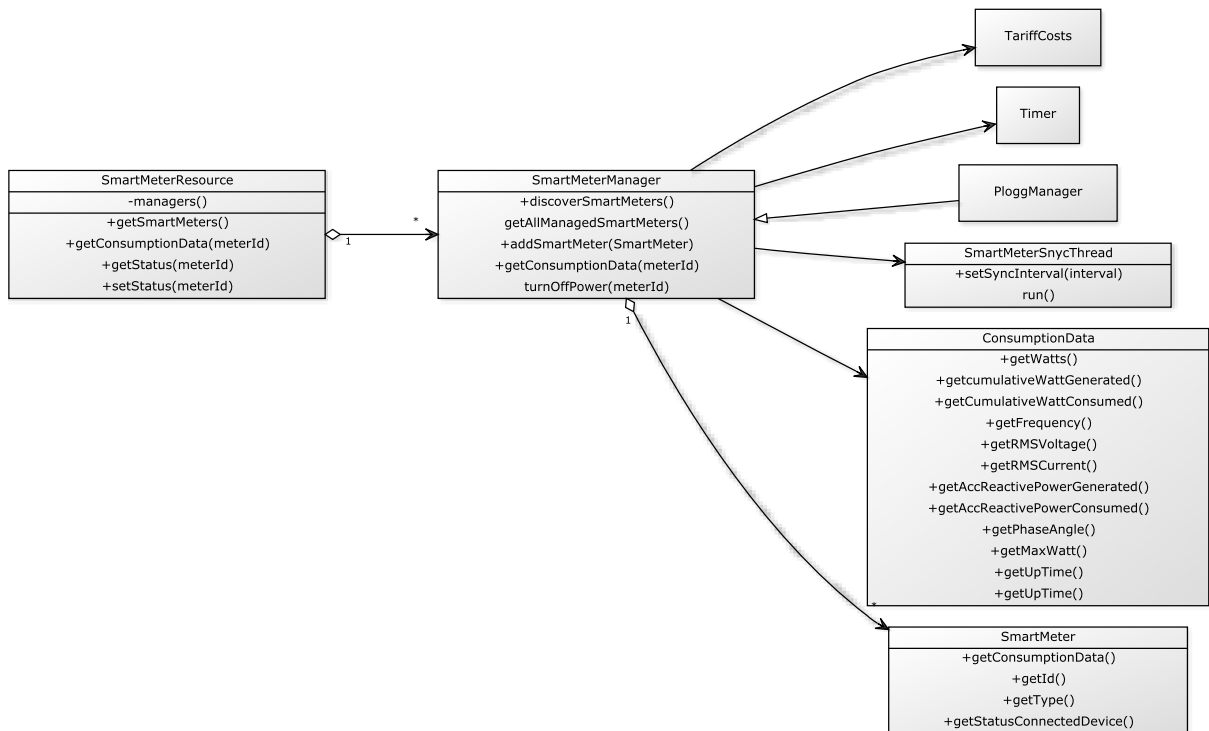
Figure 3.15: Simplified class diagram of the Webnergy framework. Concrete smart meters (e.g., Ploggs) have to extend the SmartMeterManager class. The Web representation of the smart meter data is taken care of by the SmartMeterResource .
