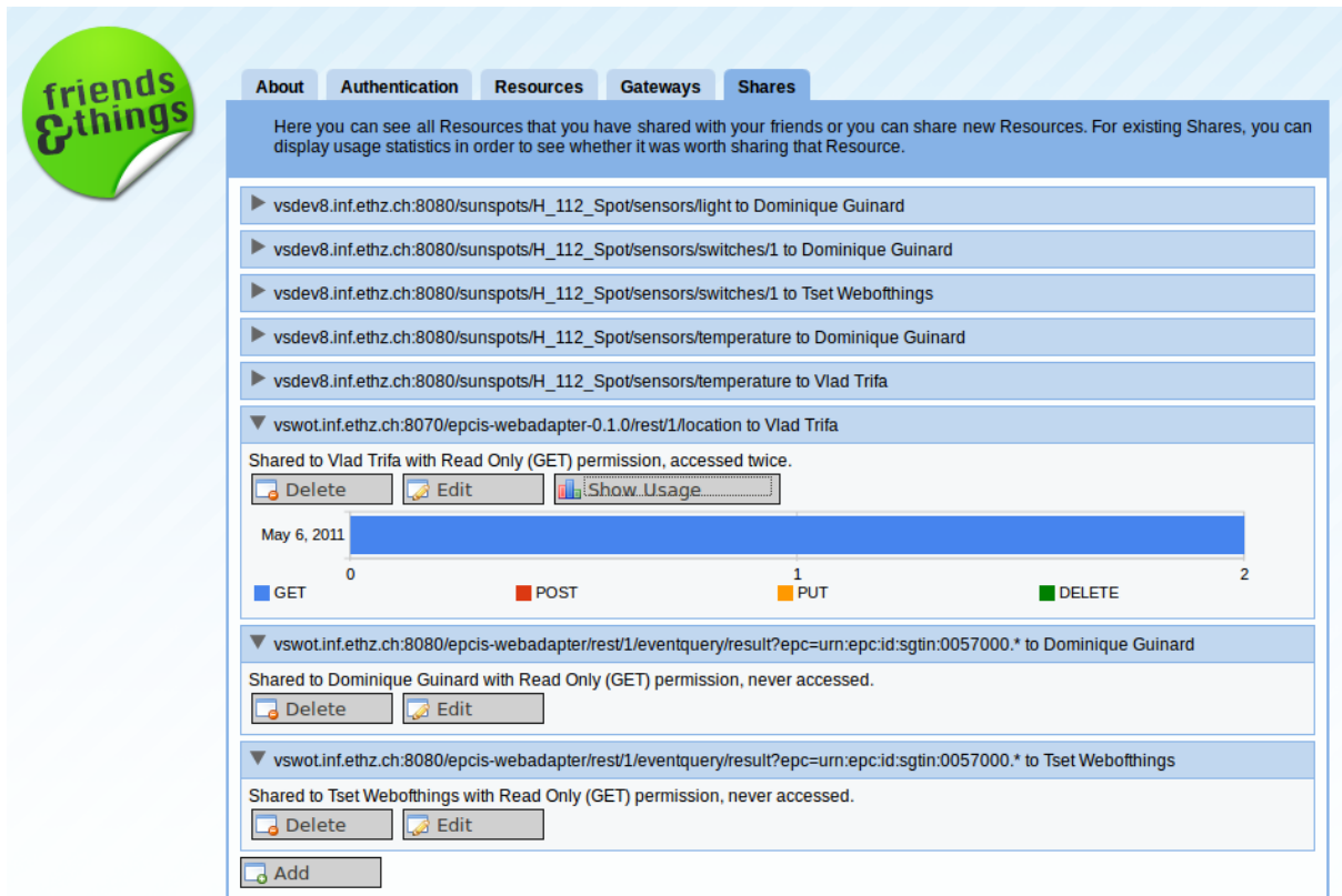
Figure 4.12: Friends and Things user interface for monitoring the resources' usage. Usage statistics for several resources are available on this page. For instance, traces of all the products from manufacturer 0057000 can be accessed by user Tset Webofthings . The displayed graph shows that user Vlad Trifa accessed the resource location twice on May 6, 2011.
