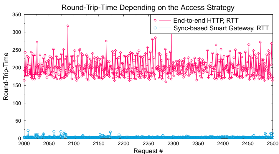
Figure 3.7: Round-trip time for 500 consecutive GET requests on a Sun SPOT node when using the end-to-end HTTP implementation and the sync-based Smart Gateway implementation (detailed in Figure 3.8).
