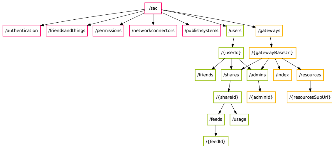
Figure 2.27: Tree visualization of the SAC RESTful Web API.
