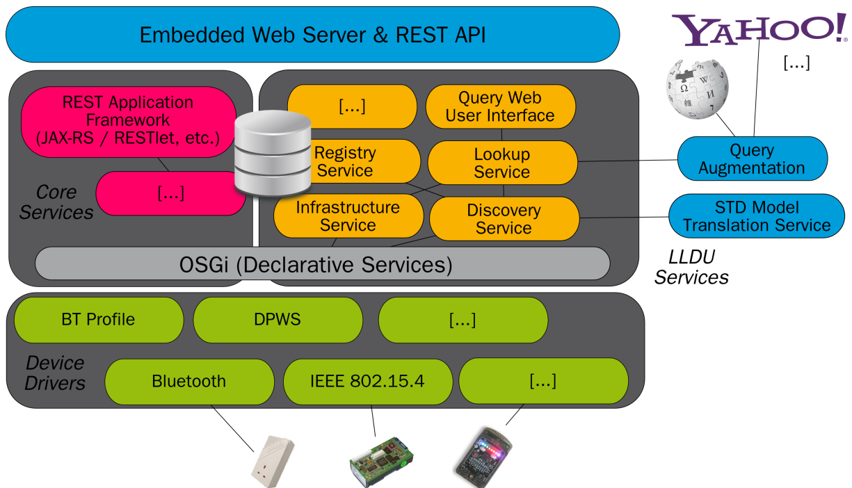
Figure 2.16: The modules of the Lookup and Discovery Infrastructure are integrated in the Smart Gateway framework through OSGi bundles. A LLDU is formed of 5 main services that are implemented as OSGi bundles running locally. Two additional services (Query Augmentation and Translation Service) can run outside the local environment (e.g., on the Web) as they can be used by several LLDUs.
