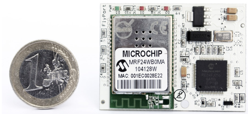
Figure 2.6: The Flyport embedded device offers a low-power WiFi module, full TCP/IP support and a native Web server supporting HTTP 1.1. (Reproduced with the kind authorization of OpenPicus, www.openpicus.com )
