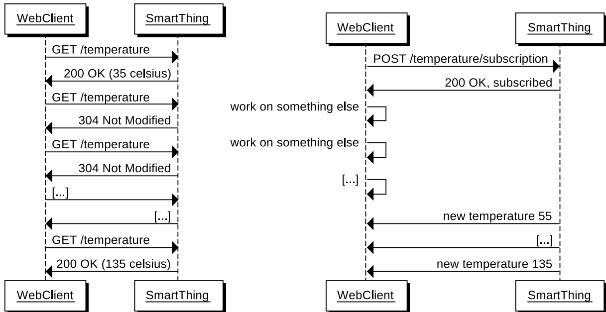
Figure 2.8: Sequence diagram of the communication between a client and a smart thing. On the left a traditional HTTP client-pull communication is started. The client has to constantly pull the smart things for updates. On the right a real-time Web approach is taken where the client is informed about the changes by the smart things.
