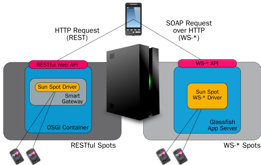
Figure 2.35: Setup of the user study. Two Sun SPOTs sensor nodes are connected to a Smart Gateway through a sync-based Device Driver (left). Their functionality is exposed through a RESTful Web API. Two other Sun SPOTs are accessible through a WS-*, SOAP + WSDL interface deployed in an application server (right).
