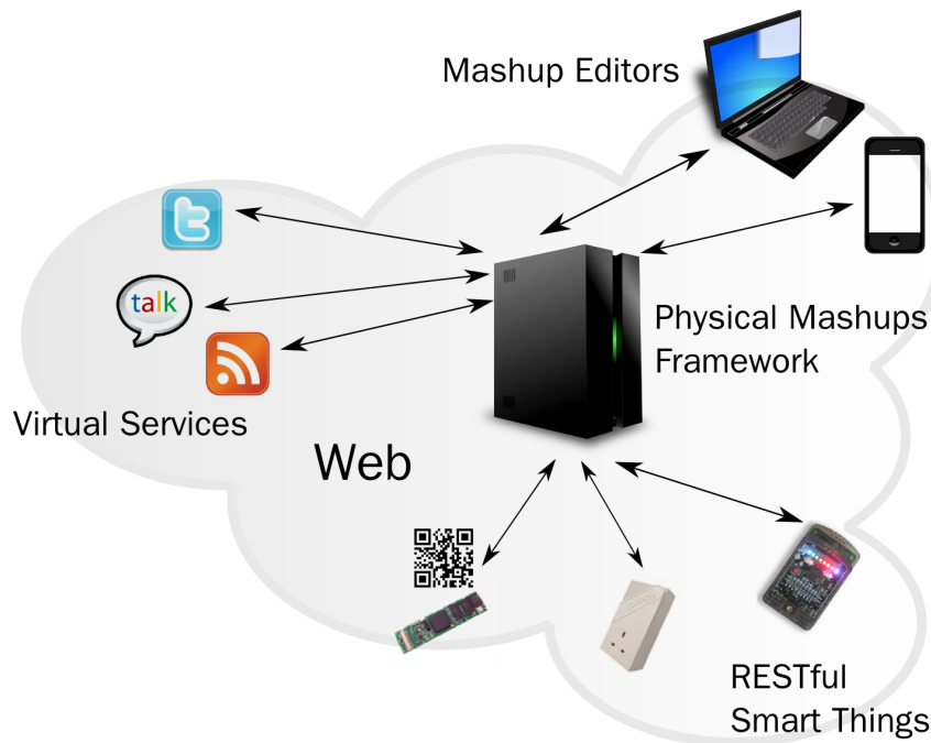
Figure 2.32: Overview of the Physical Mashups Framework. The framework is the mediator between smart things, virtual services and clients (domain-specific mashup editors).
