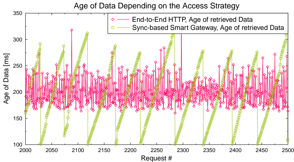
Figure 3.9: Age of the data for each request. In the HTTP end-to-end architecture the data age equals the message processing and propagation time. In the sync-based Smart Gateway the data age grows until a synchronization successfully happened.
