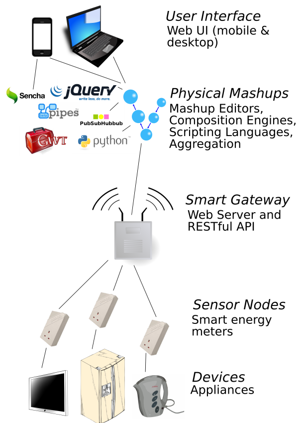
Figure 3.14: Appliances connected to Ploggs communicate with a Smart Gateway offering the Ploggs' functionality as a RESTful Web API. Physical Mashups are then built on top of the API.
