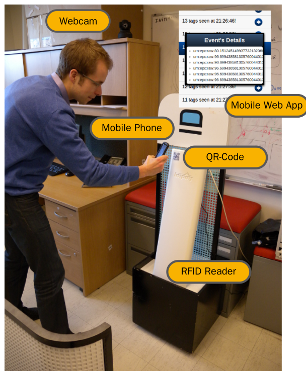
Figure 4.14: The data read by the RFID LLRP Gate reader is sent via real-time Web (Web-Sockets) to a mobile phone application running in the mobile browser. The Web application is accessed simply by scanning a QR-code.
