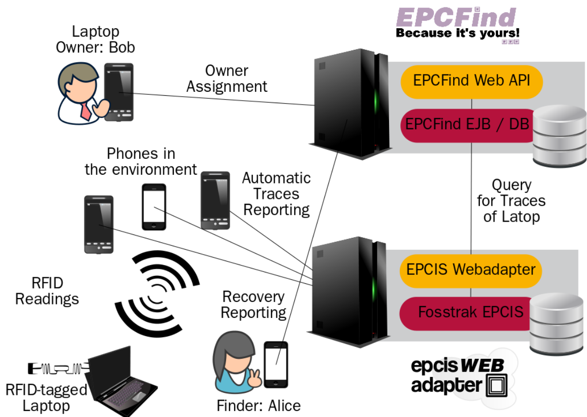
Figure 4.10: Architecture of the EPCFind prototype. Mobile phones in the environment communicate with the EPCIS Webadapter deployed on top of the Fosstrak EPCIS and record traces of tagged objects. Through the mobile EPCFind application communicating with the EPCFind backend and the EPCIS Webadapter, Bob can trace his lost laptop. It is eventually found by Alice who communicates it to the EPCFind backend and the EPCIS Webadapter.
