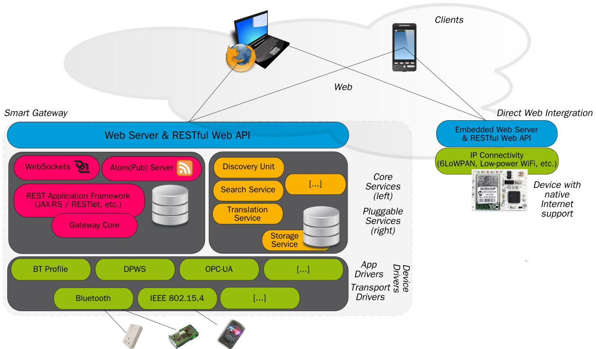
Figure 2.5: Web and Internet integration with Smart Gateways (left), direct integration (right). The Smart Gateways are small software application servers containing: Device Drivers to understand the low-level smart things, core services to create Web-APIs, pluggable services to offer additional functionality and a Web server.
