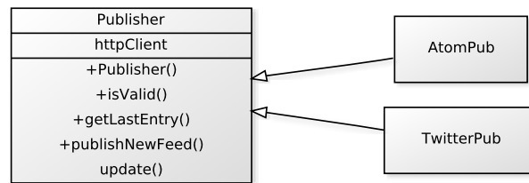
Figure 2.26: Simplified class diagram of the publishers architecture of SAC.
