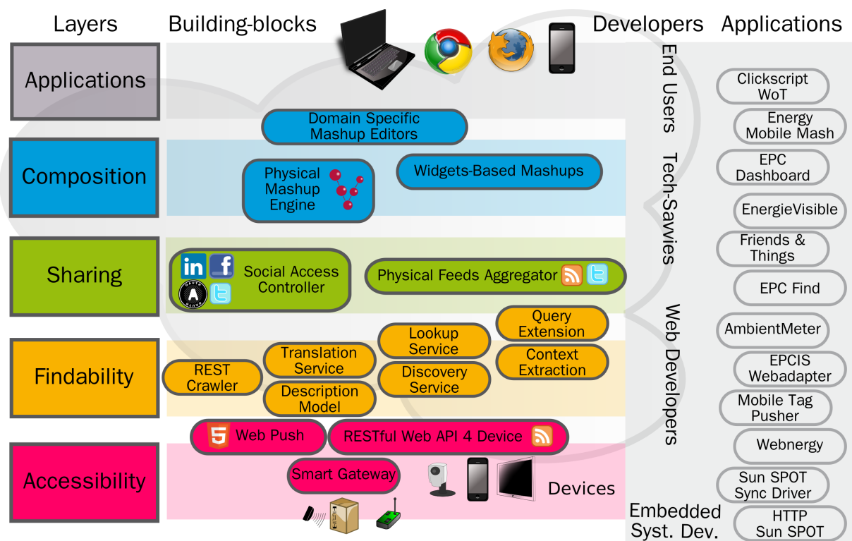
Figure 2.1: The four layers of the Web of Things architecture: Accessibility, Findability, Sharing, Composition. Applications can be built on top of each layer, but as we go up the layers they become more accessible to a broader community of developers and users. The figure provides an overview of the deliverables of this thesis. On the left-side are the architectural building-blocks. On the right-side the applications and prototypes.
