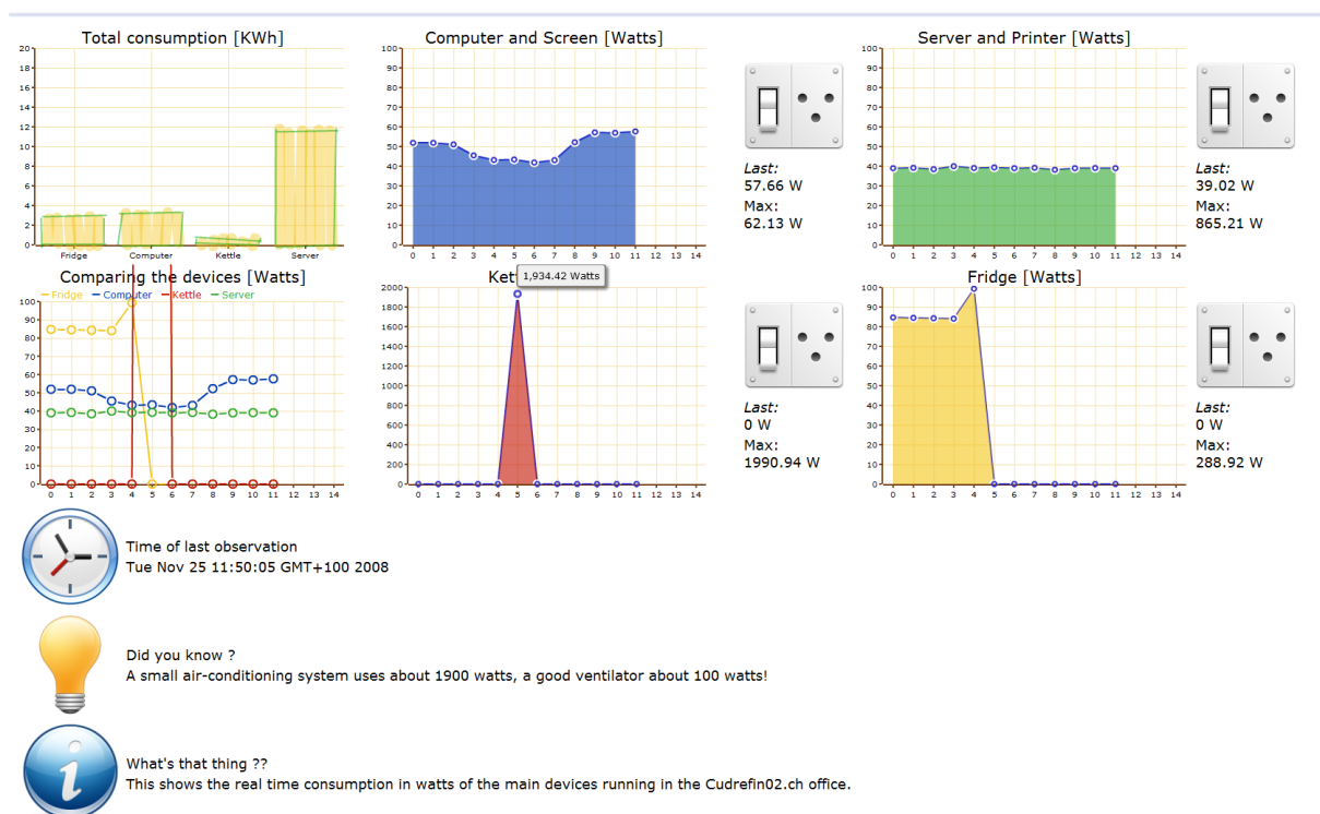
Figure 3.17: The monitoring and control Web user interface for the Ploggs shows the consumption of each connected appliance. The switch icons can be used to power on / off the devices. It is implemented as a simple JavaScript + HTML page calling the Ploggs' RESTful Web API.
