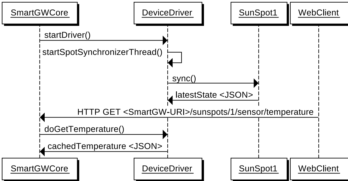
Figure 3.5: Sequence diagram of a request for the temperature of Sun SPOT 1 when using the Smart Gateway synchronization-based architecture. The Smart Gateway serves data to the clients that was cached by the DeviceDriver during the last synchronization round.
