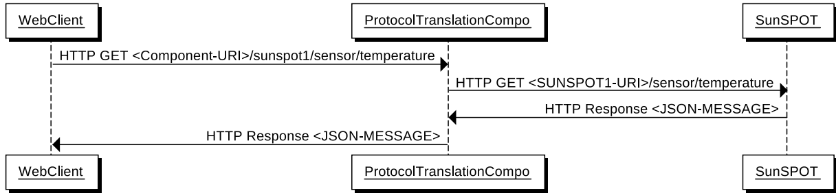
Figure 3.2: Sequence diagram of a protocol translation for the Sun SPOTs. The incoming HTTP over TCP/IP request is routed to the correct node as an HTTP request over the Sun SPOT GCF radiostream protocol (using IEEE 802.15.4).
