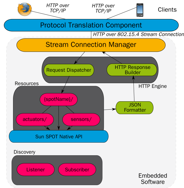
Figure 3.1: Embedded software stack directly deployed on the Sun SPOTs in order for them to natively understand the HTTP protocol. Incoming requests go through the Stream Connection Manager via the Protocol Translation component and are then sent to the Request Dispatcher. This component reads the URI and redirects the request to implementation of the corresponding resource. The resource calls the native API and sends the returned data to the JSON Formatter. The data is converted to JSON and sent back to clients.
