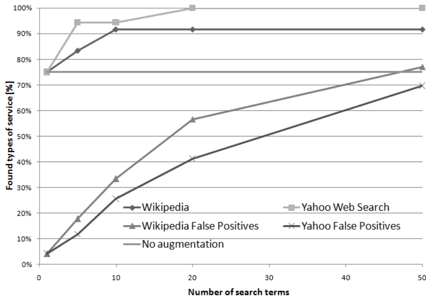
Figure 2.19: Results for the Query Augmentation with Yahoo! and Wikipedia, the Query Augmentation has a positive impact on the number of services found but it also generates more false positives.
