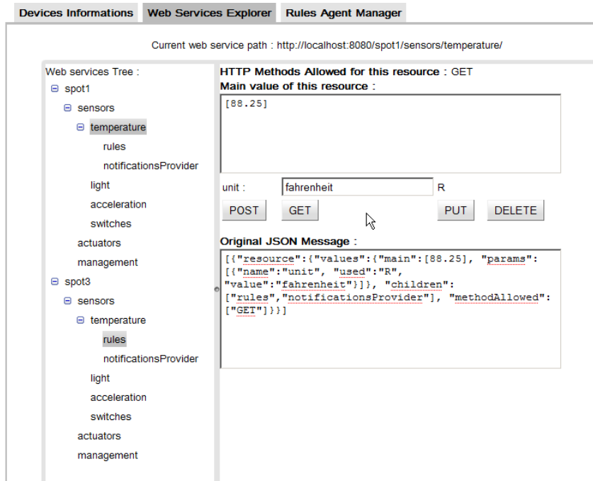
Figure 3.3: Using the AJAX ResourceExplorer, users can explore directly the resources provided by the device. This example shows how users can get the current temperature resource values and the formalism of the JSON response.
