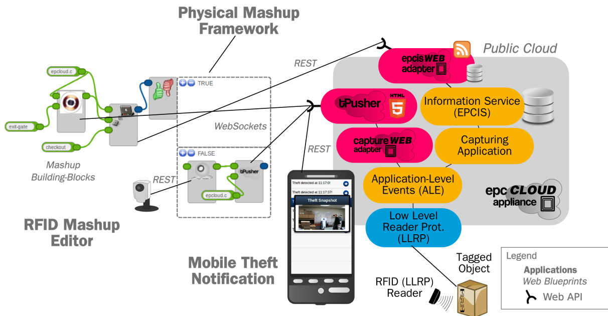
Figure 4.18: The RFID Mashup editor is used to model the EAS use-case. The created mashup can then be run from the Physical Mashups Framework. Thefts are reported to a mobile phone.
