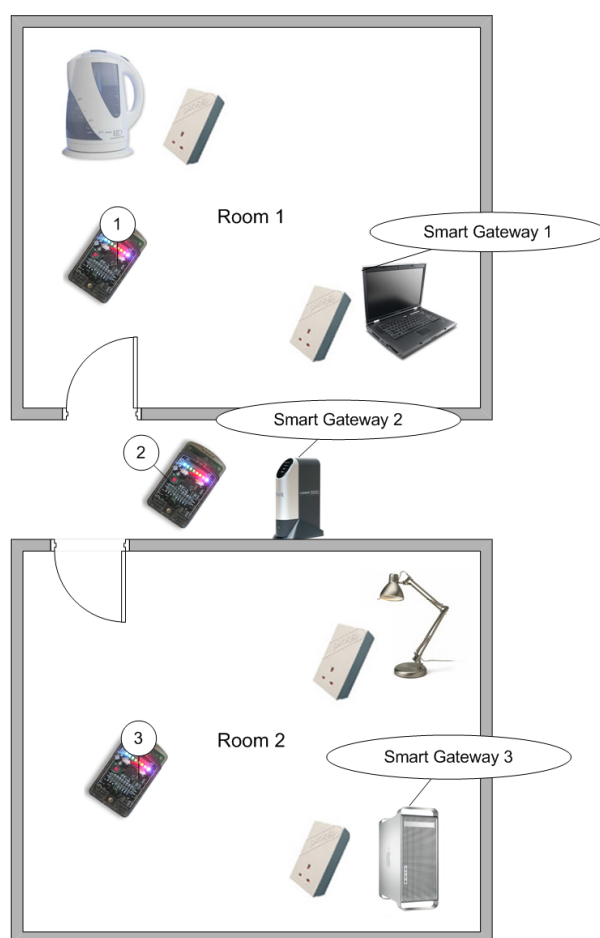
Figure 3.21: Demonstration settings of the Ambient Meter. Every 5 seconds the Ambient Meter (implemented with a RESTful Sun SPOT) polls a URI for an assessment of the energy consumption observed by all the Ploggs the Smart Gateways discovered.
