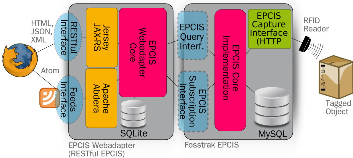
Figure 4.7: Architecture of the EPCIS Webadapter based on the Jersey RESTful framework and deployed on top of the Fosstrak EPCIS.
