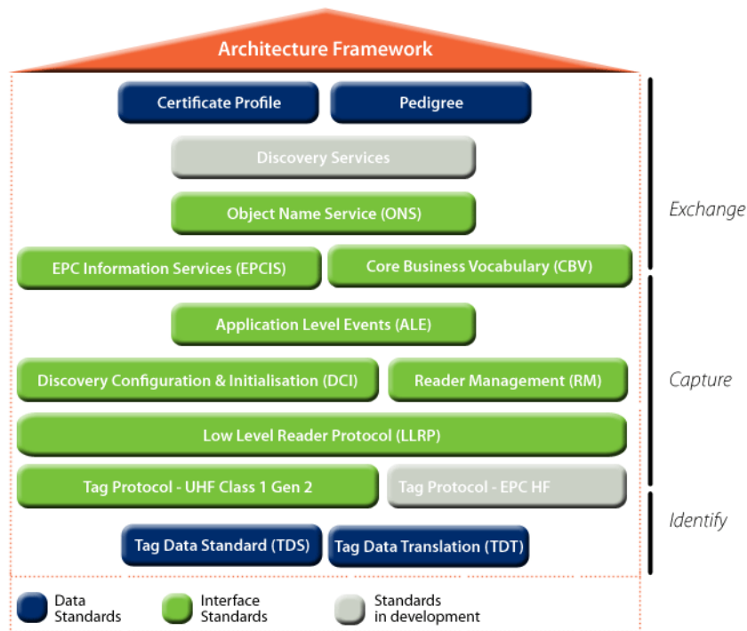
Figure 4.3: EPC Network Architectural framework composed of 14 standards (Source [189]).
