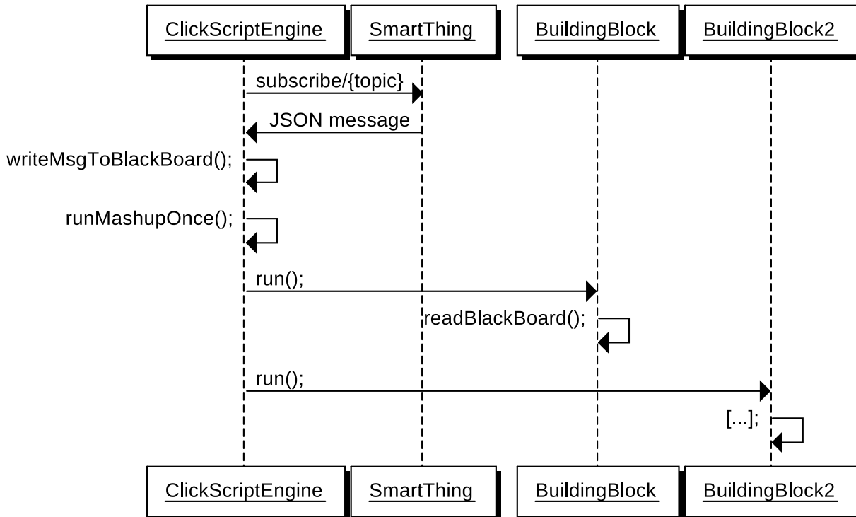
Figure 2.31: Sequence diagram of a typical Web-push triggered execution in the extended version of the Clickscript mashup editor. The editor subscribes to a WebSocket (or Comet) topic and writes the incoming messages to a black-board variable which is then read by building-blocks.
