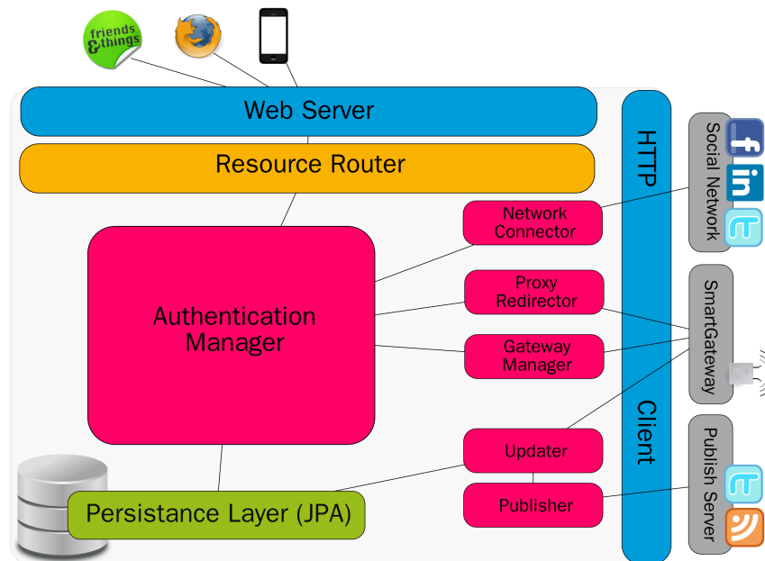
Figure 2.24: Overview of the SAC software architecture. At the core of the architecture, the AuthenticationManager is responsible for managing a list of the connected users. The NetworkConnectors are used to authenticate and authorize users with all supported social networks. The GatewayManager manages the Smart Gateways and the ProxyRedirector fetches resources from the Smart Gateways in the name of trusted connections. Finally, Updater s and Publisher s manage the feeds.
