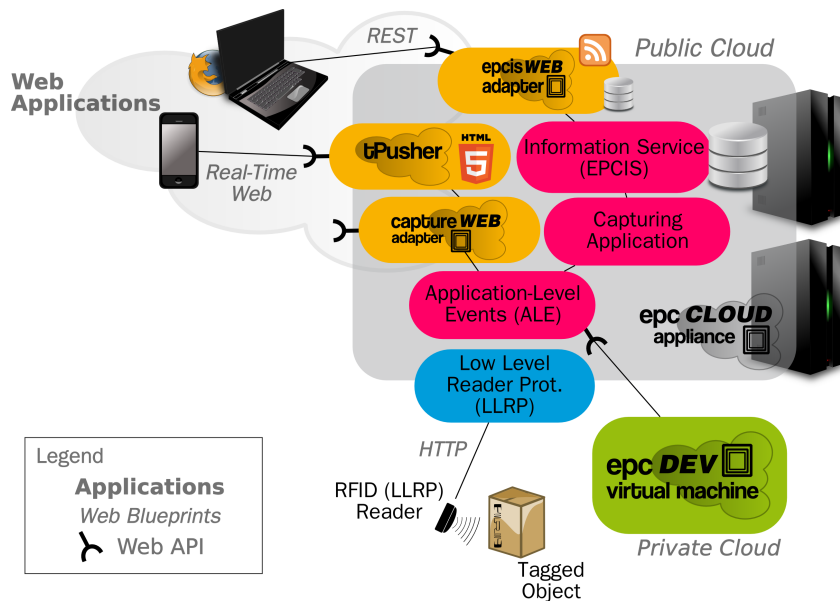
Figure 4.1: Overview of the EPC Cloud component architecture. Web components are added to the existing EPC Network components and packaged into virtual machines that can be deployed in public or private clouds. Web and mobile applications can be built on top of the new components' Web APIs.
