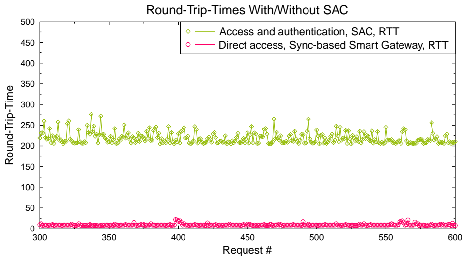
Figure 3.20: Round-trip time for 300 consecutive requests for the light resource of a Sun SPOT with or without authentication through the SAC server. The authentication process has an overhead of a about 200 ms per request.
