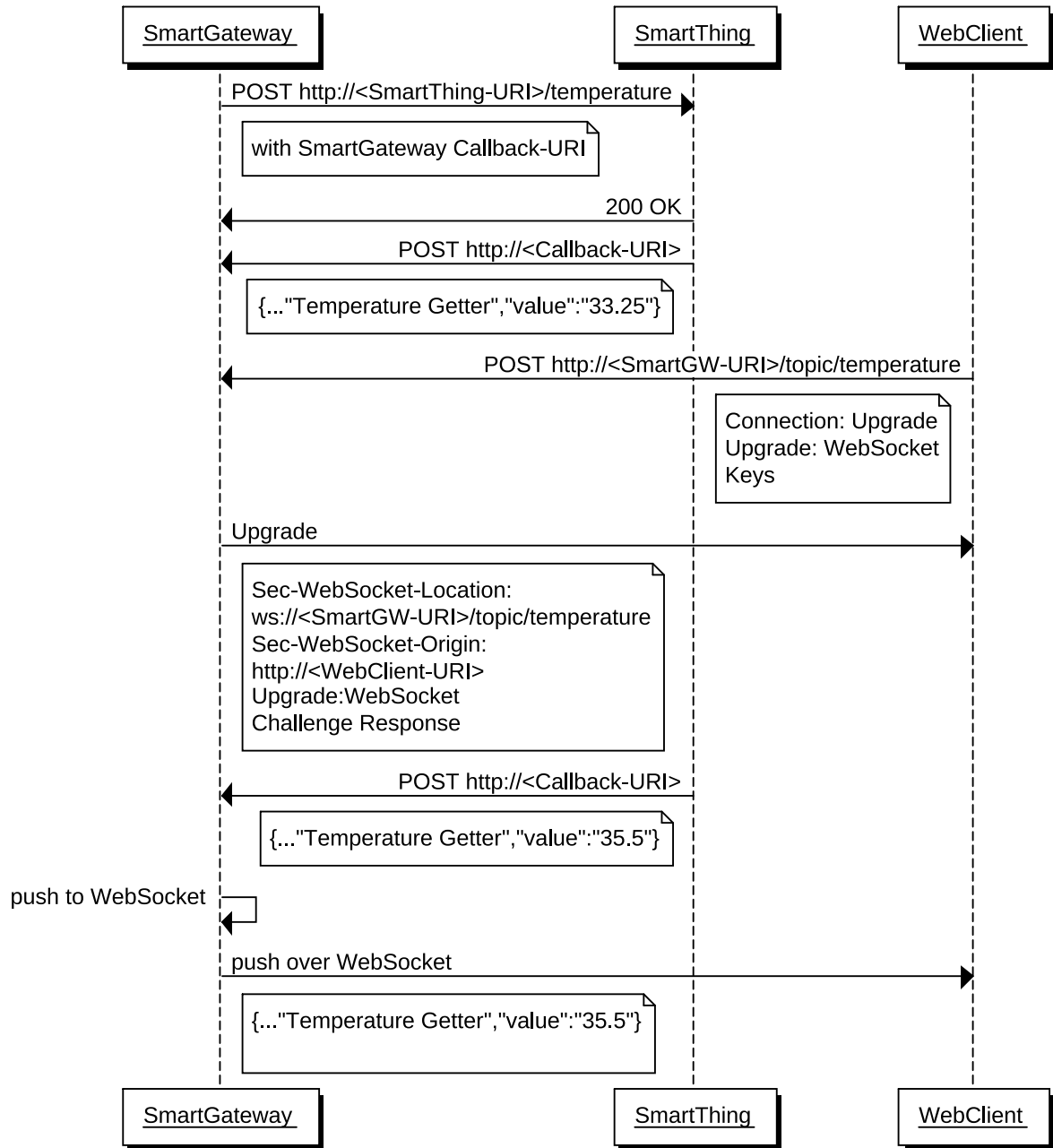
Figure 2.9: Sequence diagram of the real-time communication between Web clients and smart things through Smart Gateways and the tPusher component. tPusher is deployed on a Smart Gateway where it is used to serve content from smart things through a WebSocket interface.
