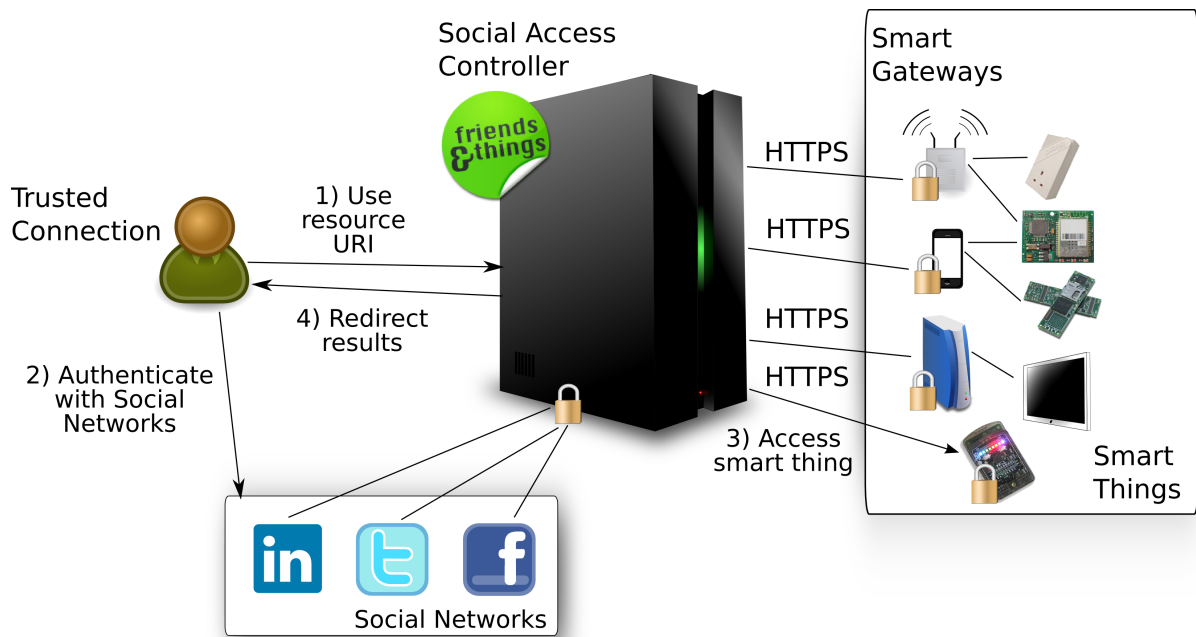
Figure 2.23: Accessing shared objects using delegated authentication through the Social Access Controller. The trusted connection requests the shared resource's URI (1). If not logged in with the corresponding social network, the SAC server asks the trusted connection to login (2). The SAC server then access the smart thing and redirects the results to the trusted connection's client (3, 4).
