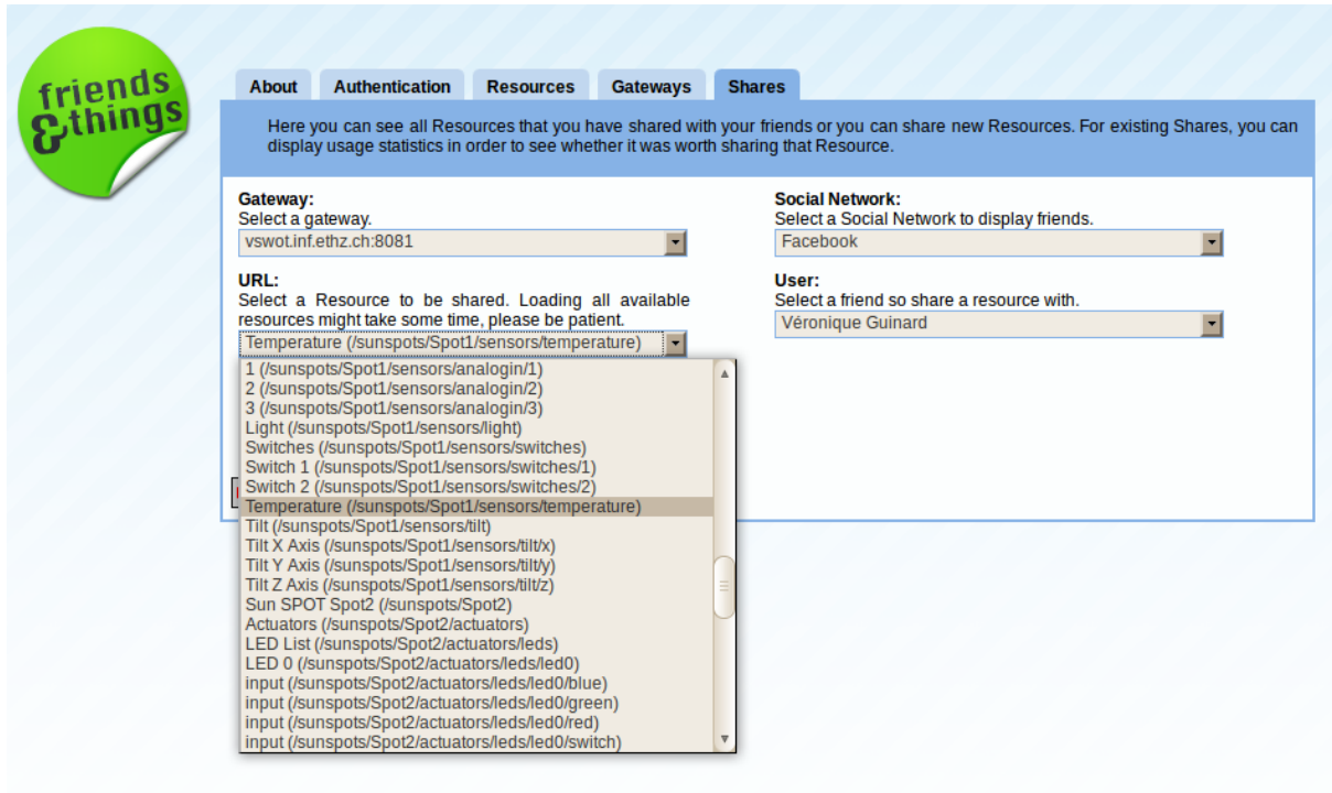
Figure 3.19: Screenshot of the Friends and Things Web user interface (built on top of the SAC API) after crawling the resources of a Sun SPOTs Smart Gateway. All resources are extracted and ready to be shared with trusted connections.
