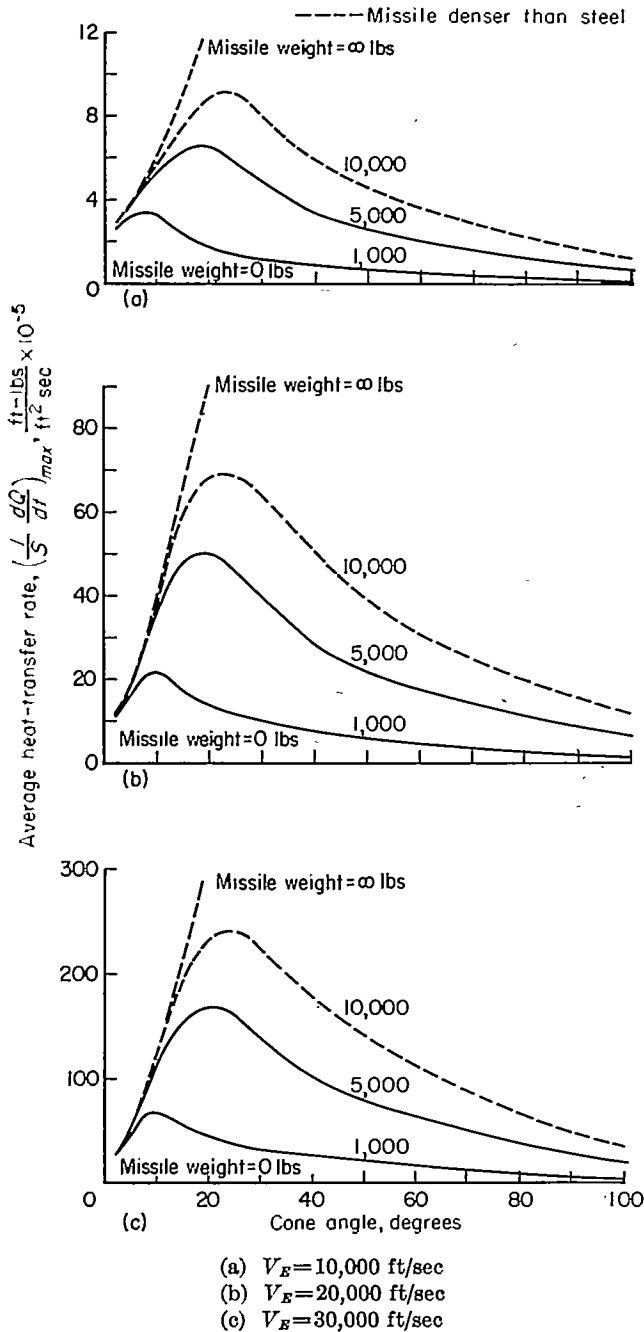
FIGURE 8.—Maximum average rate of convective heat transfer to conical missiles of the same volume entering the earth's atmosphere at an angle of 30° to the horizontal and velocities of 10,000, 20,000, and 30,000 ft/sec (volume=16.34 cu ft).
