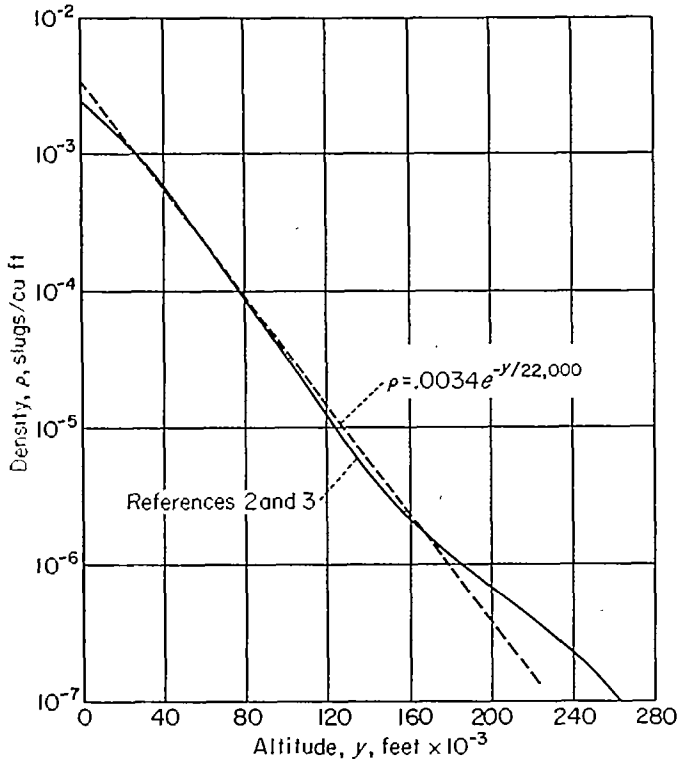
FIGURE 1.—Variation of density with altitude.
