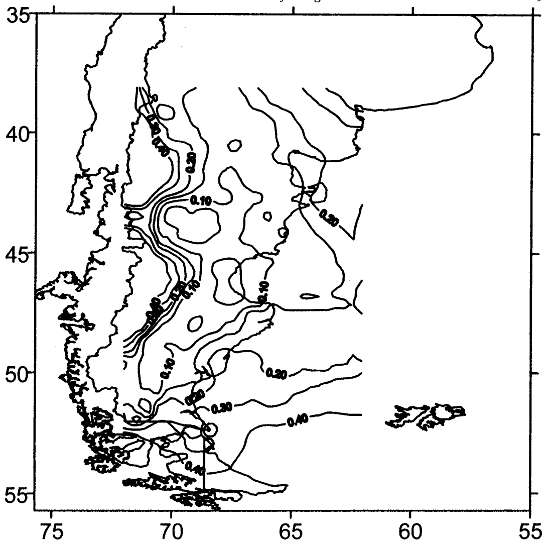
Figure 6. Aridity Index (MAP/PET) for Patagonia. MAP data corresponded to the Leemans and Cramer (1991) database. PET was calculated from mean annual temperature (Shaw et al. 1995).
