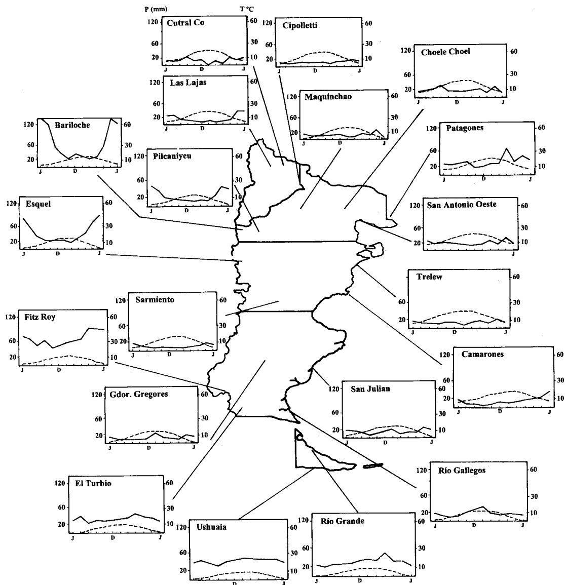
Figure 2. Seasonal distribution of precipitation and temperature for different sites in Patagonia. The solid line corresponded to monthly precipitation and the broken line to temperature.
