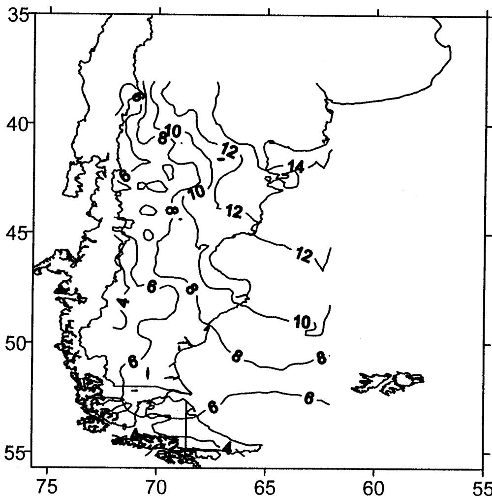
Figure 4. Mean annual temperature (MAT) of Patagonia. Data corresponded to the Leemans y Cramer (1991) database. This database has a spatial resolution 0.5 \times 0.5 of latitude and longitude. (See Paruelo et al. 1995 for a description of the database).
