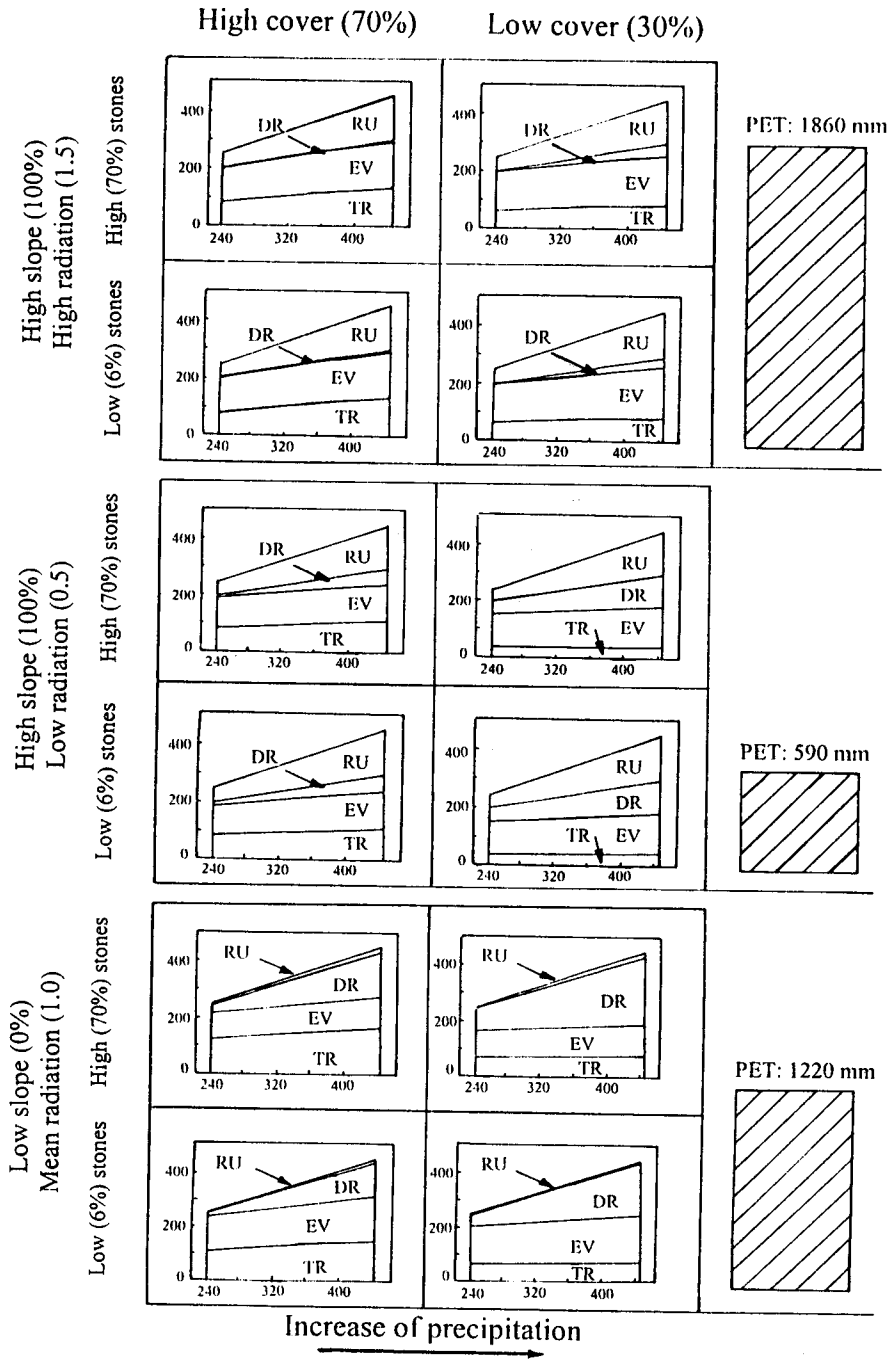
Figure 9. Transpiration (TR), Evaporation (EV), Drainaje (DR), Runoff (RU) and Potential Evapotranspiration (PET) simulated by DINAQUA (Paruelo and Sala 1995) for environmental conditions representatives of western Chubut. Each graph represent different combinations of plant cover, % stones, radiation, and slope levels.
