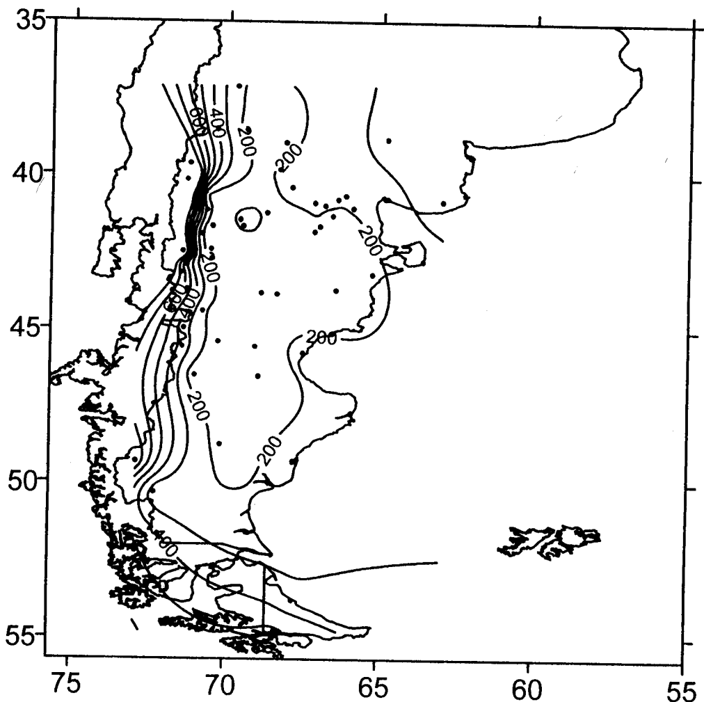
Figure 3. Mean annual precipitation (MAP) of Patagonia. Isolines were generated from 62 sites spread across the region. A list of the weather station is available at www.ifeva.edu.ar/coiron .
