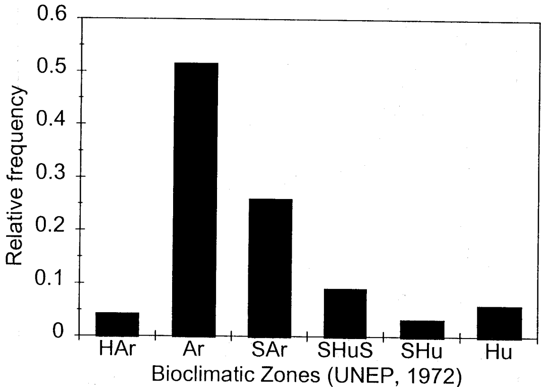
Figure 7. Proportion of Patagonia corresponding to the different bioclimatic zones defined Le Houérou (1996), on the basis of the MAP/PET ratio: Hyperarid (HAr) < 0.05 , Arid (Ar) 0.05-0.20 , Semiarid (SAr) 0.20-0.45 , Dry subhumid (SHuS) 0.45-0.65 , Subhumid (SHu) 0.65-0.75 and Humid (Hu) > 0.75 . Mean annual precipitation and temperature data corresponded to the Leemans and Cramer (1991) database. PET was calculated from mean annual temperature (Shaw et al. 1995).
