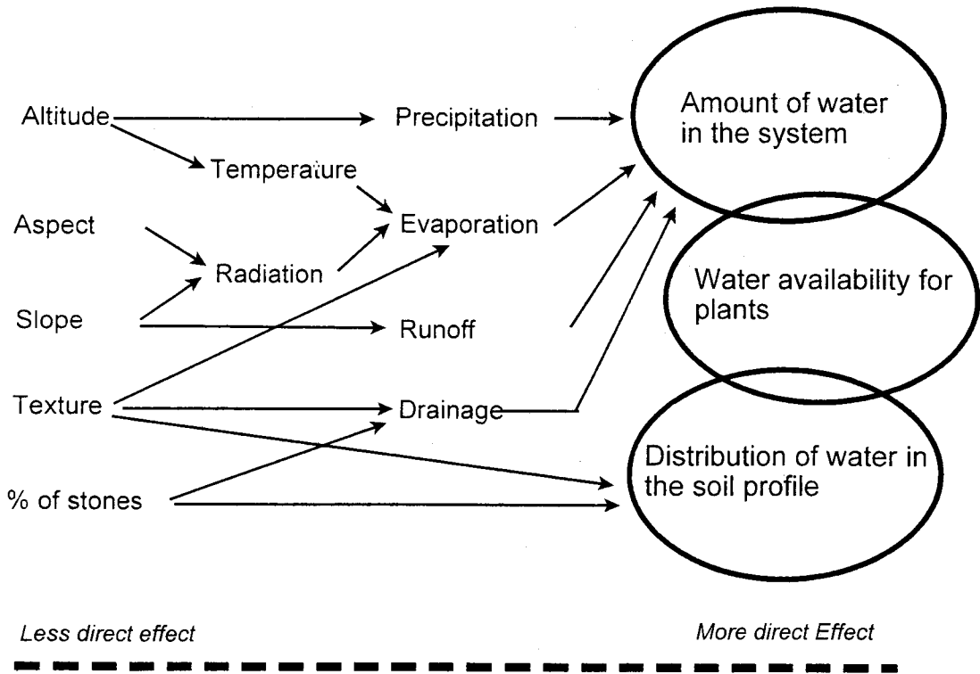
Figure 8. Influences of environmental variables on plant water availability
