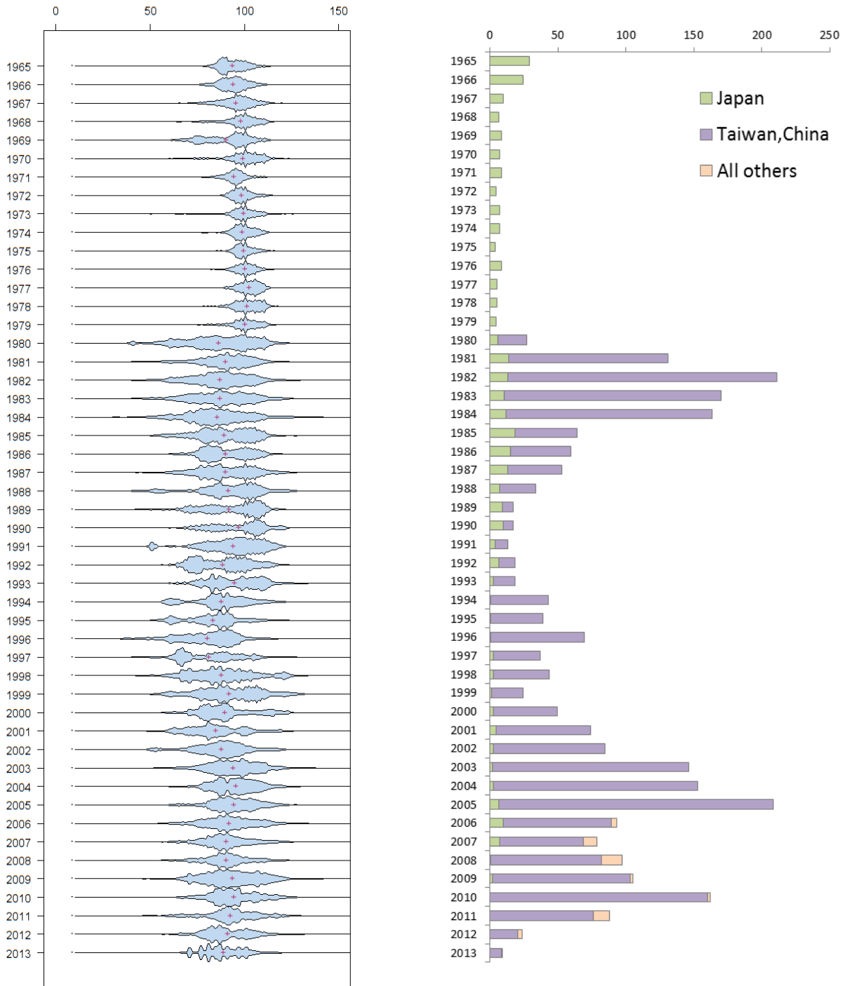
Fig. 8. Albacore: Left - Length frequency distributions (total amount of fish measured by 1 cm length class) derived from the data available at the IOTC Secretariat for freezing longline fisheries, by year. Right - Number of specimens sampled for lengths by main longline fleet.
