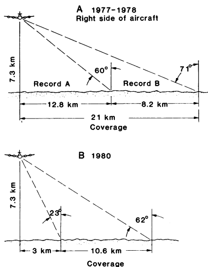
Fig. 2. Radar acquisition geometry.
