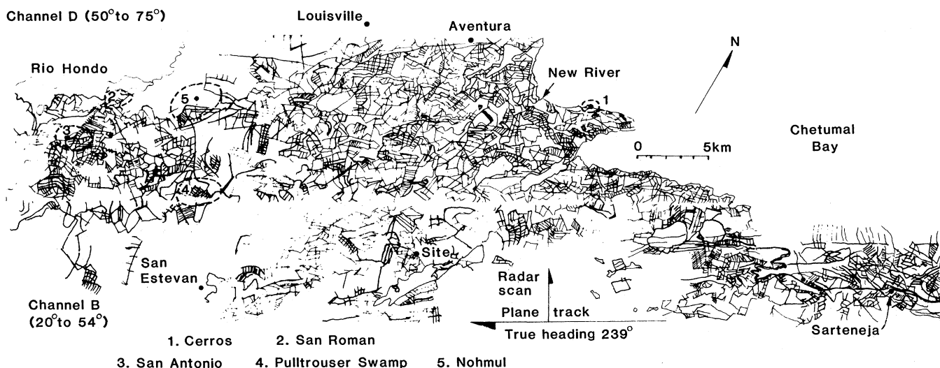
Fig. 4. Overlay of northern Belize, transcribed from radar imagery, showing the lattice structure of canal lines and the five zones where the existence of canals has been confirmed by checks.
