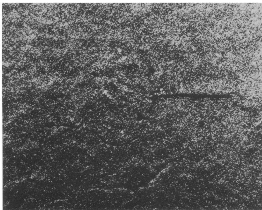
Fig. 3. Synthetic-aperture radar imagery of the Tikal zone, Guatemala. The heavy, dark horizontal line (right, center) is the Tikal airstrip. True north is 23° east of vertical. The main ruins show as a set of bright dots about 1 inch to the left of the west end of the airstrip. The Temple of the Inscriptions shows below and slightly to the left of the airstrip and in the loop of a road that leads up to the airstrip. Depression angle of the radar was 23° to 62°. Scale about 1:75,000.
