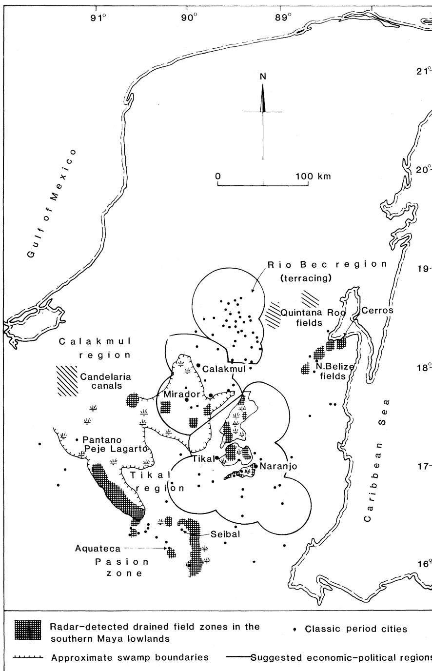
Fig. 1. Map of the Maya lowlands showing drained field zones detected by radar in relation to known Maya cities of the southern and intermediate areas.
