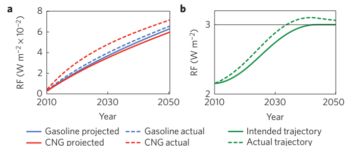
Figure 2 | \text{GWP}(100) underestimates the radiative forcing contribution of \text{CH}_4 -emitting technologies. a , The actual radiative forcing (RF) impacts of satisfying constant US passenger vehicle energy demand with gasoline versus compressed natural gas (CNG) differ from \text{GWP}(100) -based projections, with a greater discrepancy for CNG due to its higher \text{CH}_4 intensity. b , A hypothetical situation is shown (based on scenario C in Fig. 3a), in which global transportation emissions are replaced by emissions from a technology with the \text{CH}_4 intensity of CNG, using the \text{GWP}(100) to determine \text{CO}_2 equivalence (Supplementary Section 1.2). This results in a significant deviation from the intended radiative forcing scenario.
