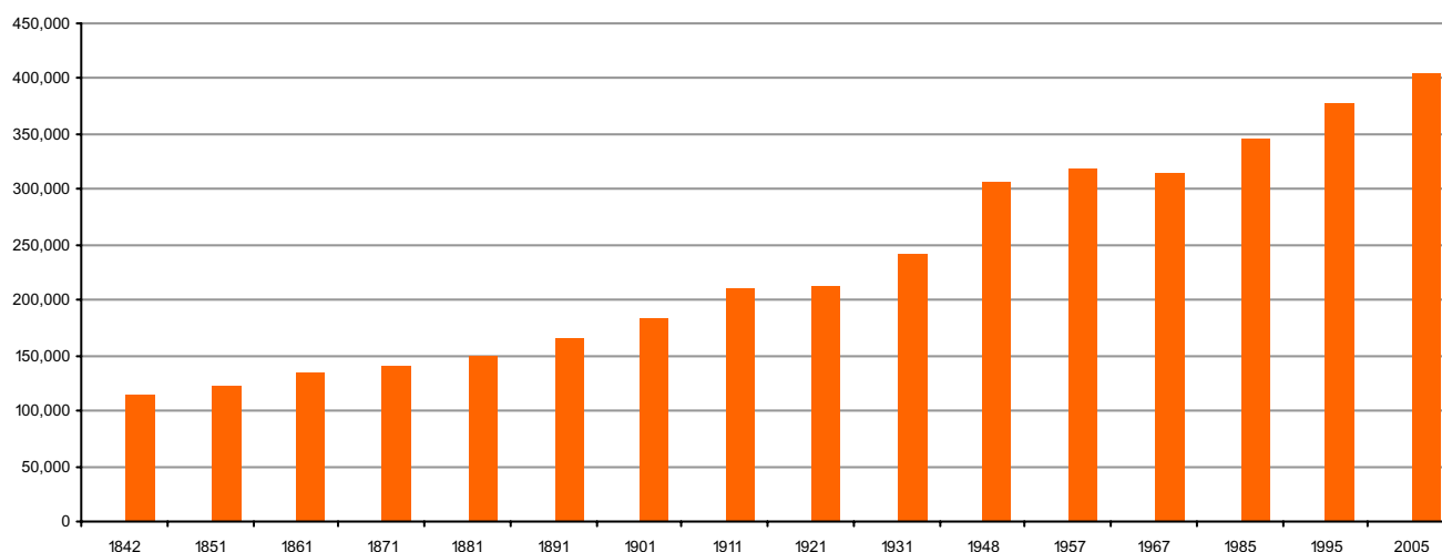
C1. Population: 1842-2005
