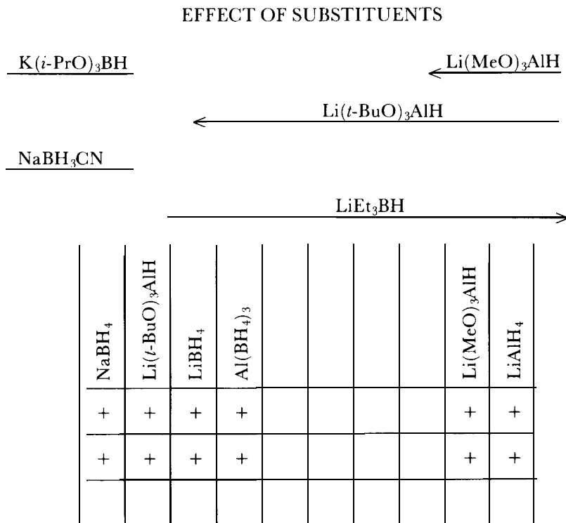
Fig. 2. Alteration of the reducing power of the two extreme reagents, sodium borohydride and lithium aluminum hydride.
