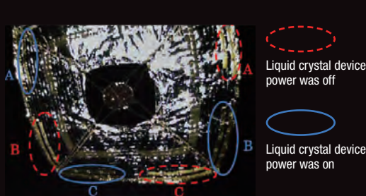
Image taken by DCAM1 confirms that the liquid crystal devices are operating properly
