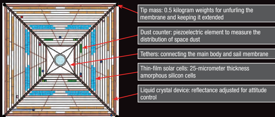
Membrane: 7.5-micrometer thickness polyimide resin with aluminium vapor deposited on one side; reinforced to prevent splitting
