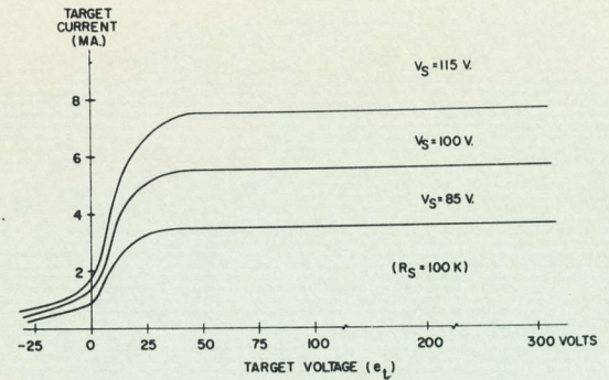
Figure 4 Output characteristic
