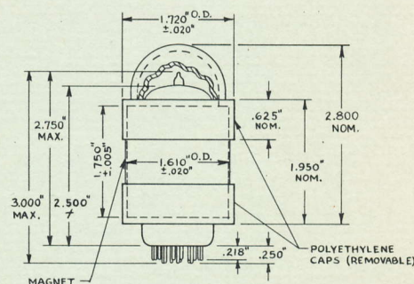
Figure 1 Outline Drawing
