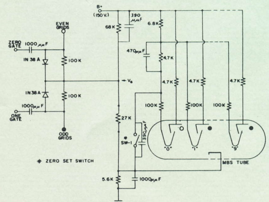
Basic Circuit for 6700
