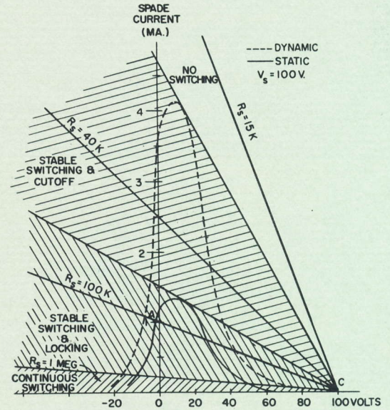
Figure 5 Beam Forming & Locking Spade Characteristic
