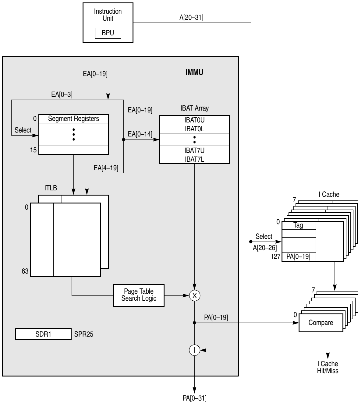
Figure 5-2. PowerPC Broadway Microprocessor IMMU Block Diagram
