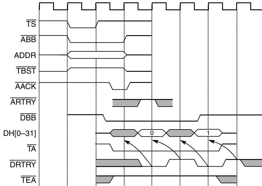
Figure 8-23. 32-Bit Data Bus Transfer (Two-Beat Burst with DRTRY)
