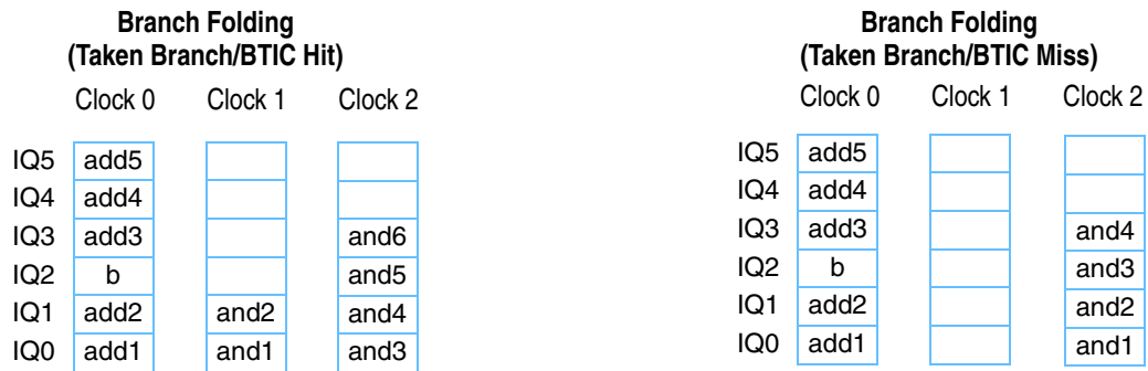
Figure 6-7. Branch Taken
