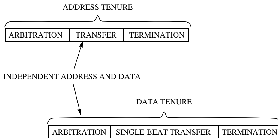
Figure 8-4. Overlapping Tenures on the Broadway Bus for a Single-Beat Transfer
