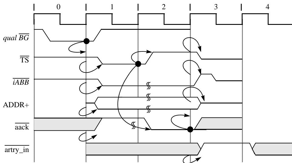
Figure 8-7. Address Bus Transfer
