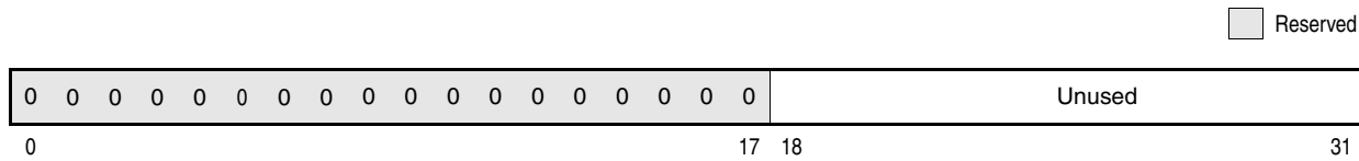
Figure 2-13. Thermal Management Register 3 (THRM3)
