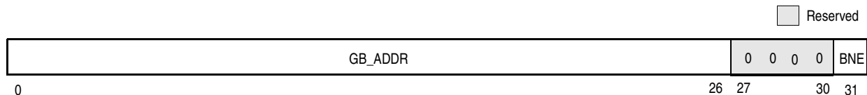
Figure 2-19. Write Pipe Address Register (WPAR)
