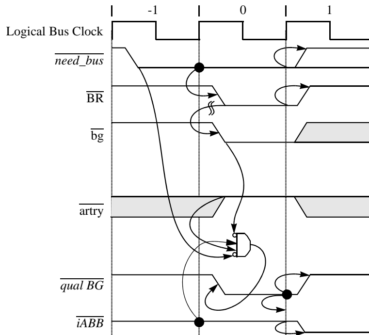
Figure 8-5. Address Bus Arbitration
