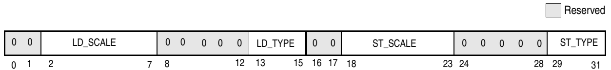
Figure 2-18. Graphics Quantization Register
