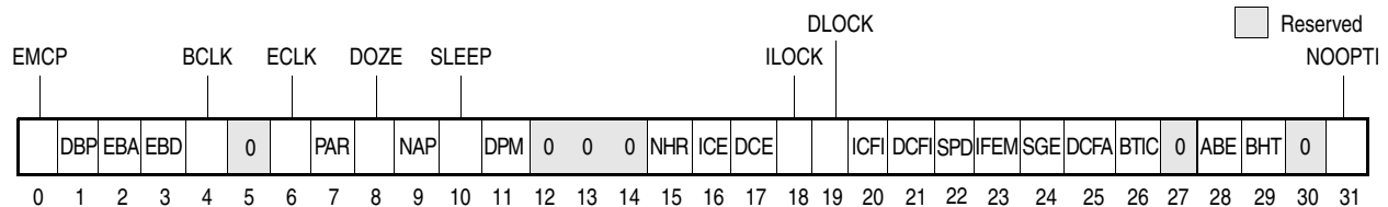
Figure 2-3. Hardware Implementation-Dependent Register 0 (HID0)
