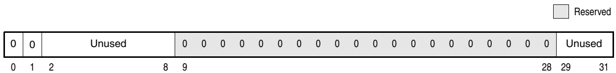
Figure 2-12. Thermal Management Registers 1–2 (THRM1–THRM2)
