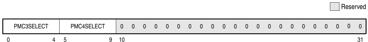
Figure 2-8. Monitor Mode Control Register 1 (MMCR1)
