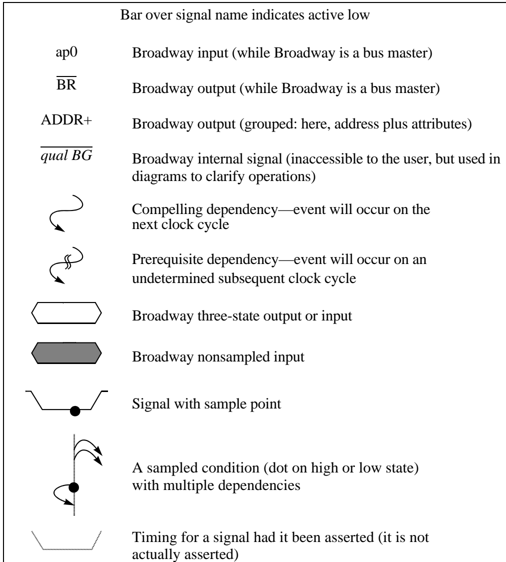
Figure 8-3. Timing Diagram Legend
