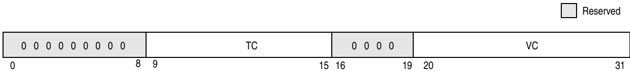
Figure 2-15. TDCH Register
