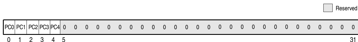
Figure 2-4. Hardware Implementation-Dependent Register 1 ( \text{HID1} )
