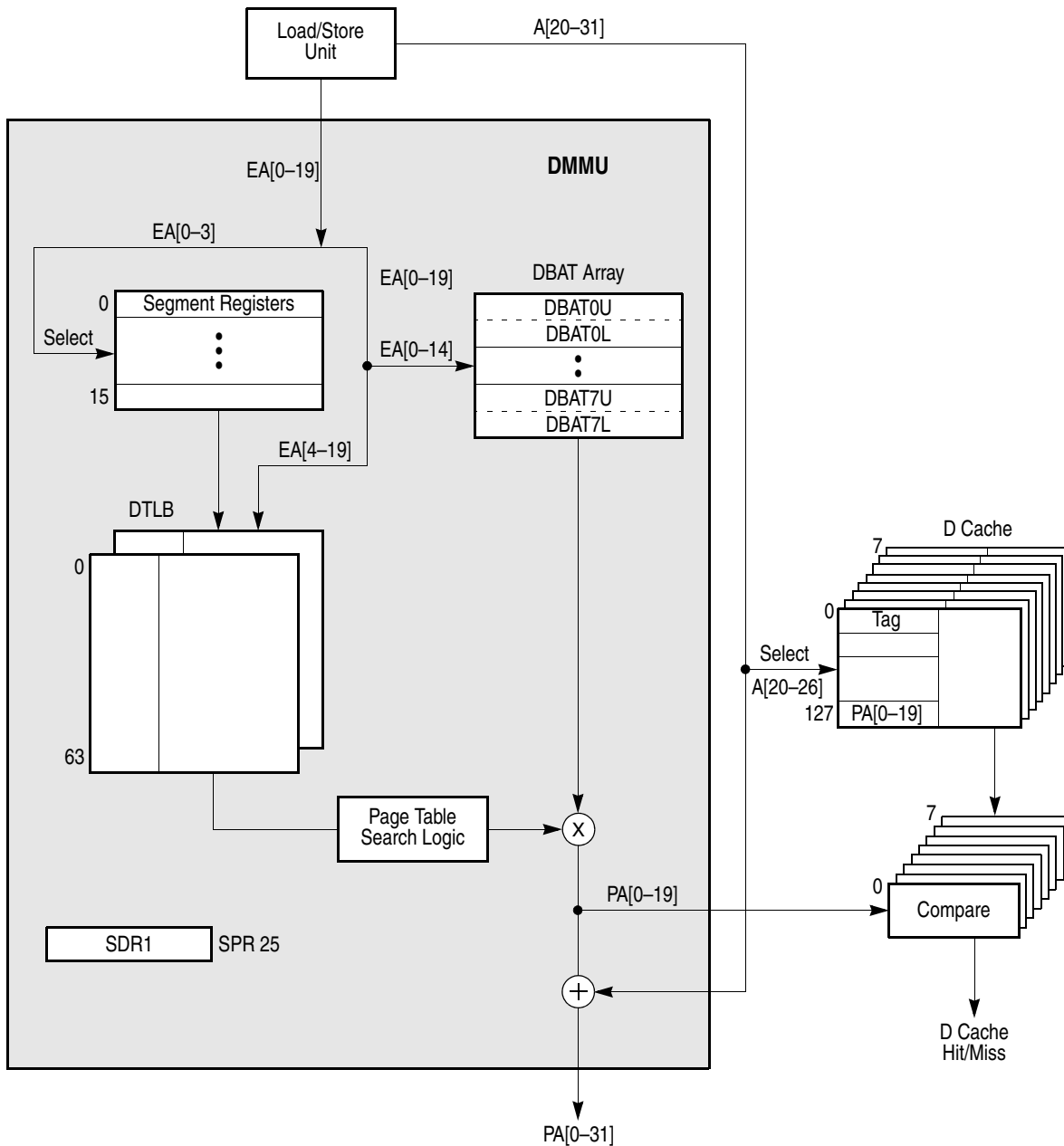
Figure 5-3. Broadway Microprocessor DMMU Block Diagram
