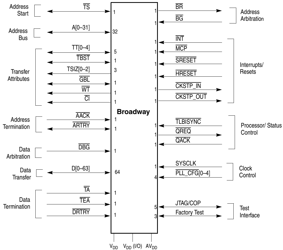
Figure 7-1. PowerPC Broadway Signal Groups
