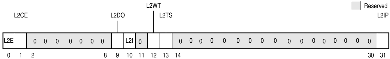
Figure 2-20. L2 Cache Control Register (L2CR)
