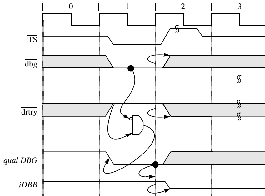
Figure 8-9. Data Bus Arbitration
