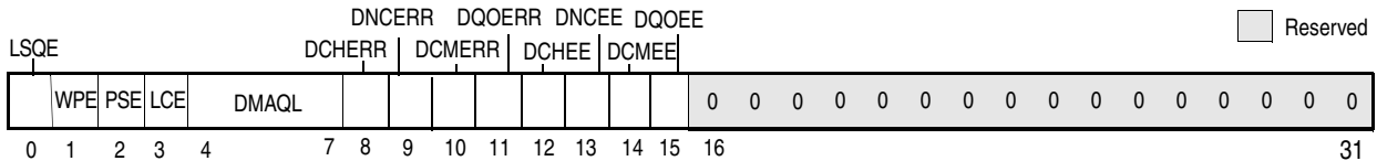
Figure 2-5. Hardware Implementation-Dependent Register 2 (HID2)
