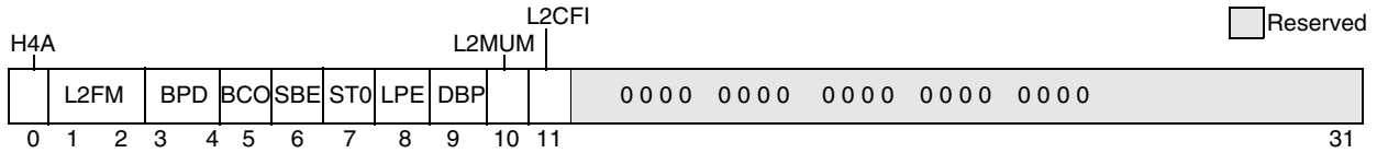
Figure 2-6. Hardware Implementation-Dependent Register 4 (HID4)
