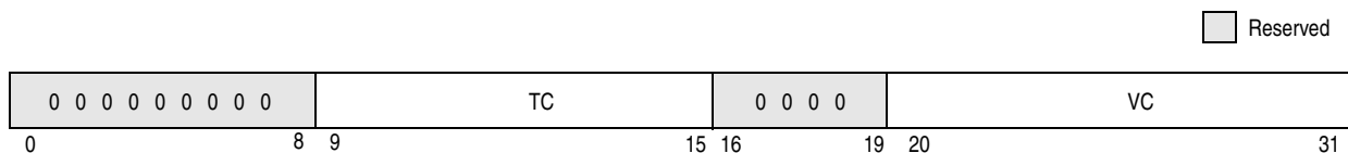
Figure 2-14. TDCL Register
