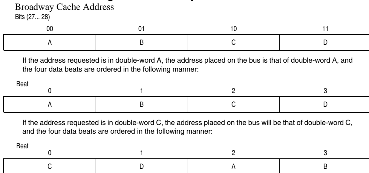
Figure 3-6. Broadway Cache Addresses
