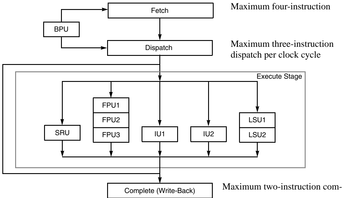
Figure 1-3. Pipeline Diagram
