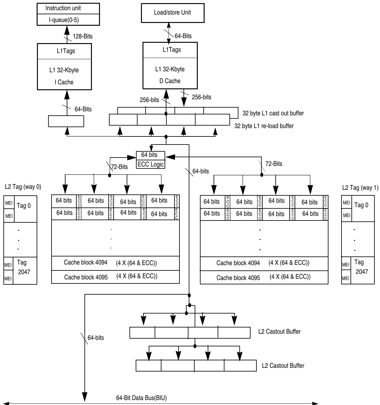
Figure 9-1. L2 Cache
