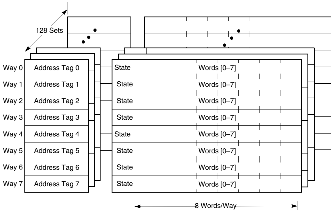
Figure 1-1. Cache Organization
