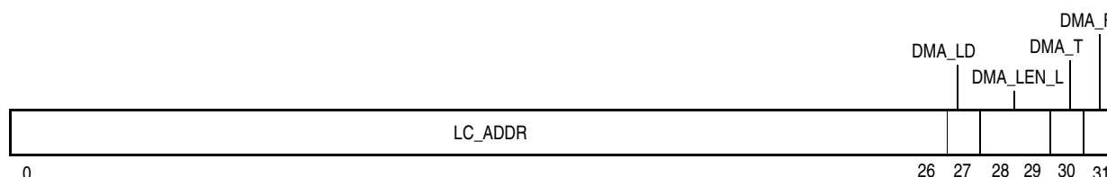
Figure 2-17. Direct Memory Access Lower (DMAL) register
