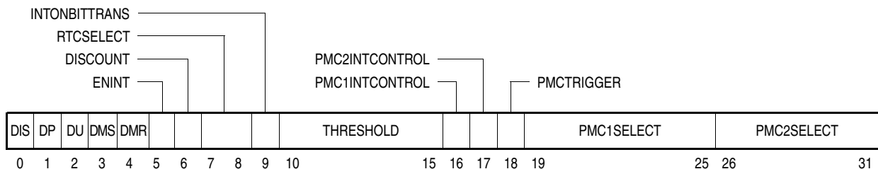
Figure 2-7. Monitor Mode Control Register 0 (MMCR0)
