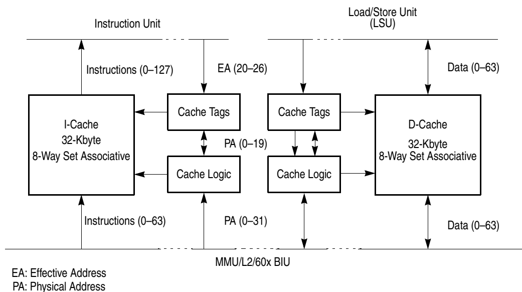
Figure 3-1. Cache Integration
