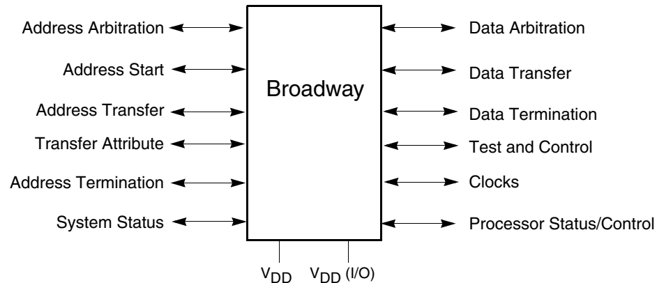
Figure 1-2. System Interface
