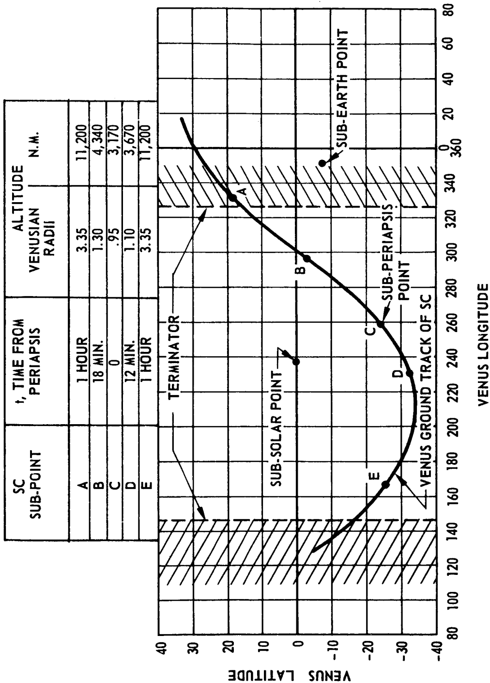
FIG. 2-7 GROUND TRACK OF FLYBY TRAJECTORY
