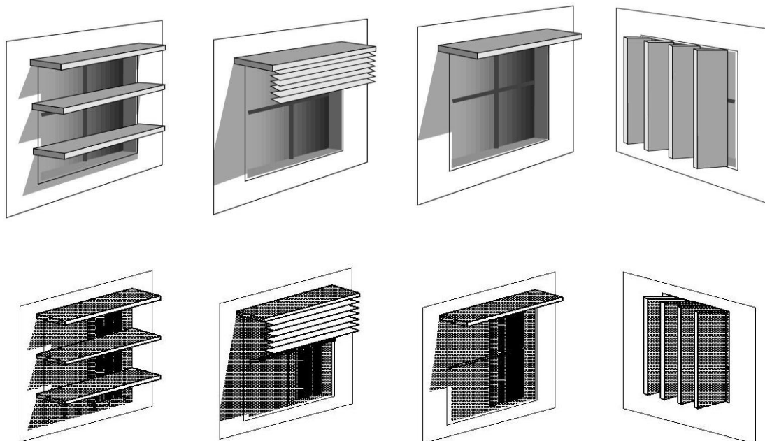
FIG. 10 COMMONLY USED SHADING DEVICES
