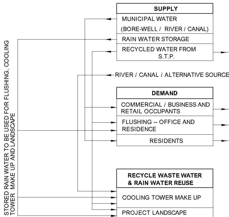
FIG. 16 TYPICAL SCHEME SHOWING GENERAL COMPONENTS OF WATER MANAGEMENT SYSTEM
