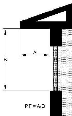
FIG. 6 PROJECTION FACTOR FOR HORIZONTAL OVERHANG
