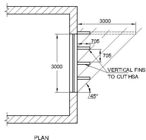
FIG. 12 DESIGN OF SHADING DEVICE TO CUT HSA
