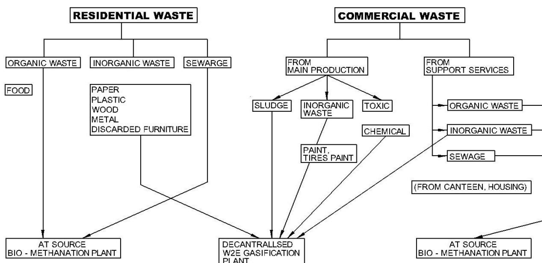
FIG. 17 TYPICAL SCHEMATIC DIAGRAM INDICATING SOLID WASTE MANAGEMENT SYSTEM
