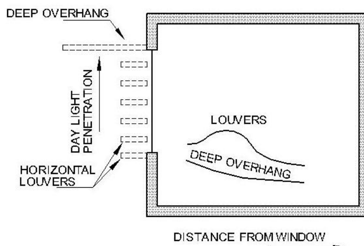
FIG. 13 COMPARISON OF DAYLIGHT PENETRATION WITH USE OF TWO SHADING DEVICES NAMELY DEEP OVERHANGS AND LOUVERS
