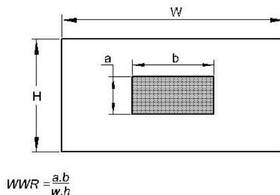
FIG. 4 WINDOW WALL- AREA
