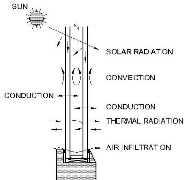
FIG. 5 TYPICAL FLOW OF SOLAR HEAT AND AIR INFILTRATION
