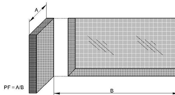
FIG. 7 PROJECTION FACTOR FOR VERTICAL FIN
