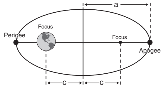
Figure 6-15. Elliptical geometry. (Adapted from Air University, Space Primer , unpublished book, 2003, 8-11.)
