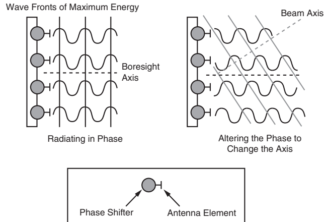
Figure 19-2. Changing direction of beam in phased-array radar. (Adapted from University of Wisconsin Naval ROTC, "Naval Weapons Systems Lesson 7: Electronic Scanning and Phased Array Radars," course files.)
