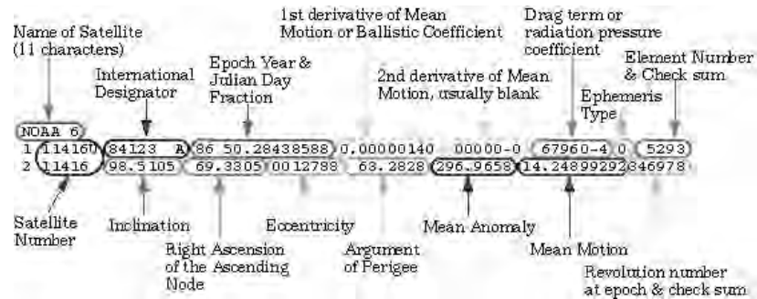
Figure 6-21. TLE set format. (Reprinted from NASA, “Definition of Two-Line Element Set Coordinate System,” Human Space Flight Web site, http://spaceflight.nasa.gov/realdatasightings/SSApplications/Post/JavaSSOP/SSOP_Help/tle_def.html [accessed 18 April 2008]).
