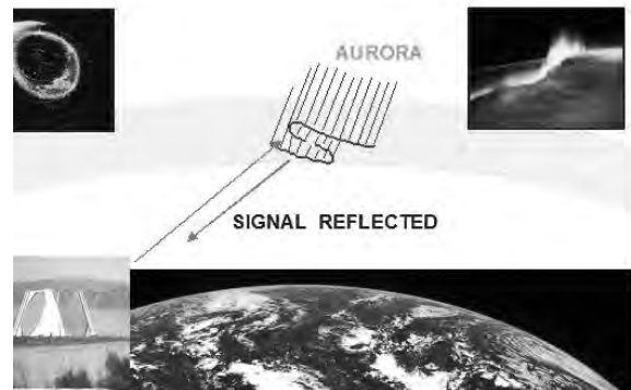
Figure 7-9. Radar aurora. (Reprinted from Air University, Space Primer , unpublished book, 2003, 6-10.)
