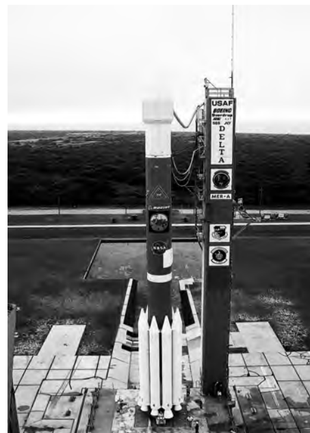
Figure 20-1. Delta II launch. (NASA photo)
