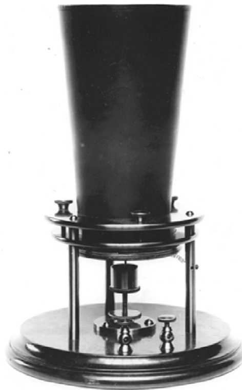
Bell's original liquid transmitter microphone
