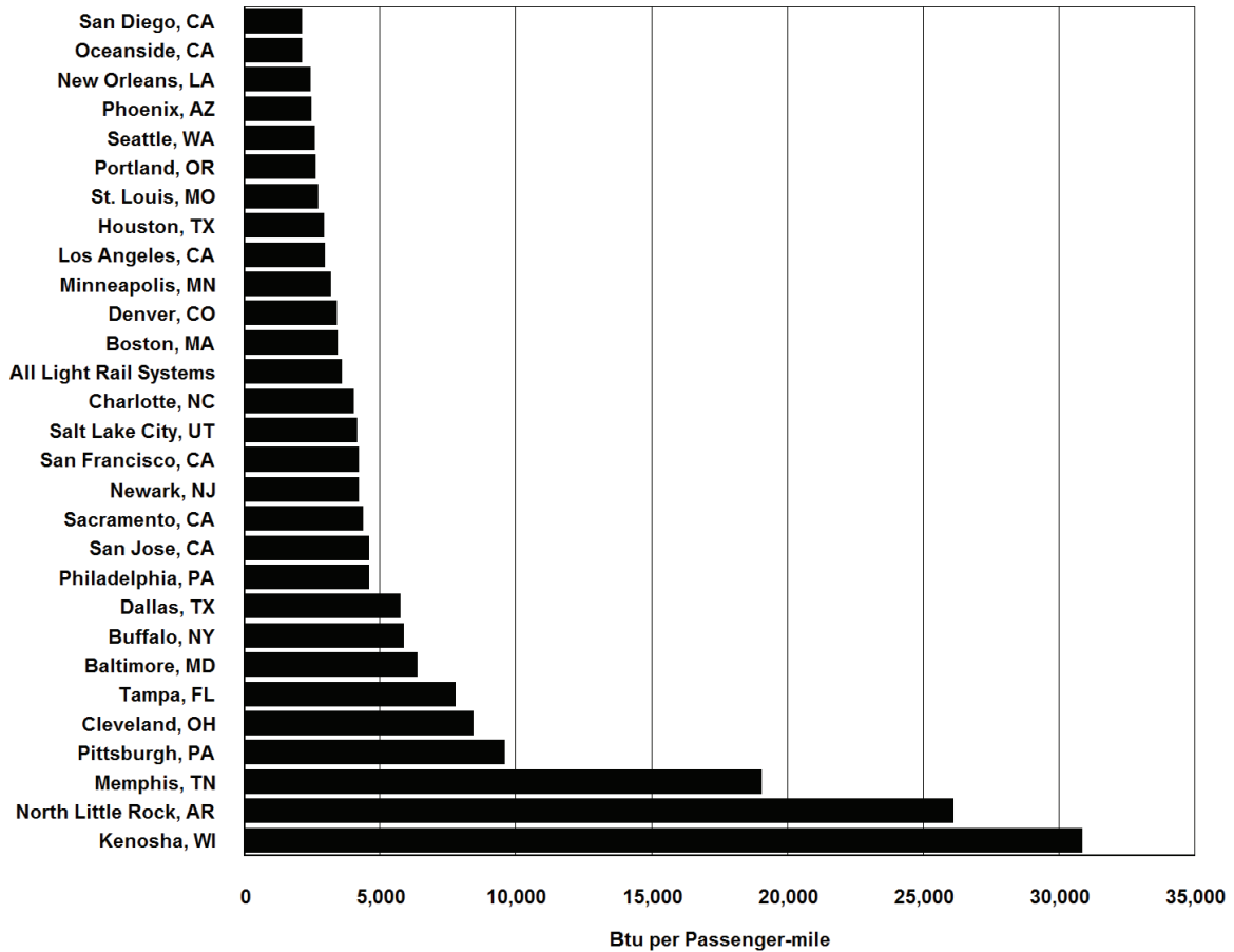
Figure 2.2. Energy Intensity of Light Rail Transit Systems, 2010
