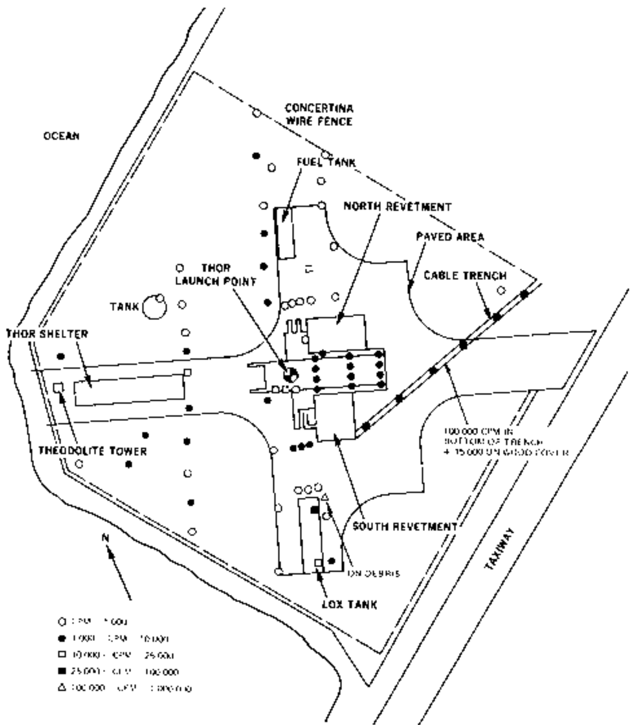
Figure 97. Thor launch pad contamination levels after 2 weeks of decontamination efforts, DOMINIC (source: Reference C.2052).
