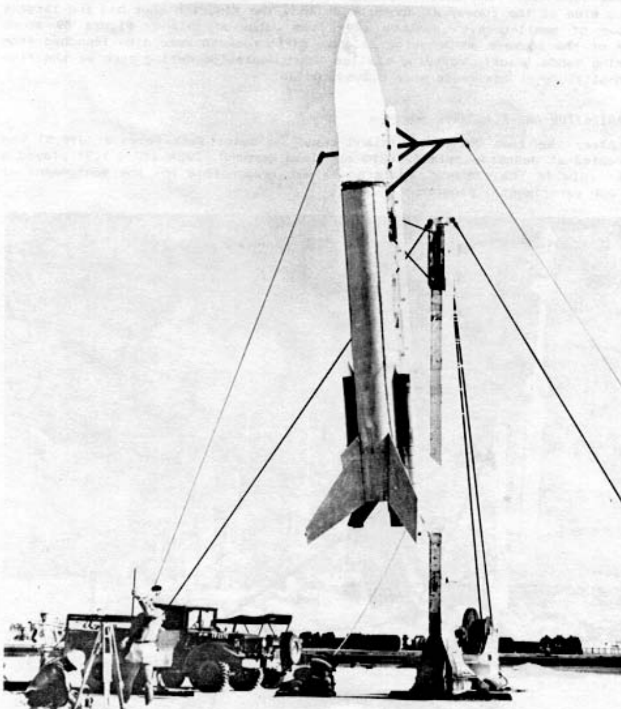
Figure 88. Stryx missile with Recruit boosters used for CHECKMATE shot, Operation DOMINIC.
