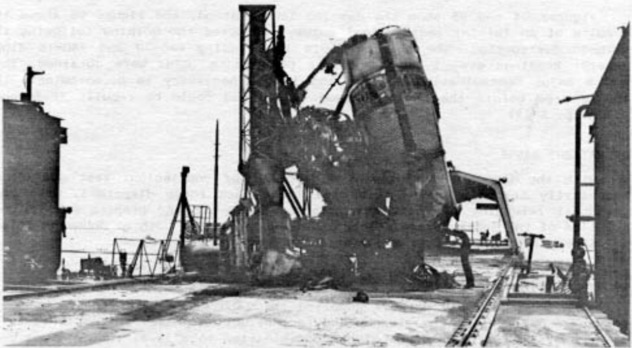
Figure 94. Thor pad after BLUEGILL Prime fire, Johnston Island, Operation DOMINIC. Compare with Figure 85 from nearly same point of view.
