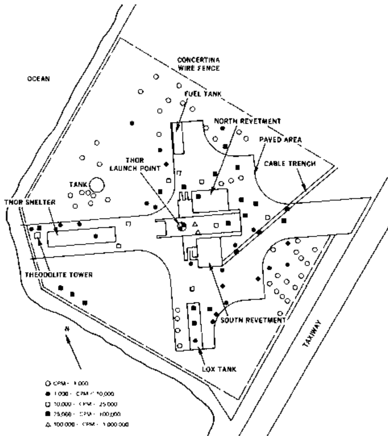
Figure 96. Initial radiological survey of the Thor launch pad following DOMINIC, BLUEGILL Prime (source: Reference C.2052).
