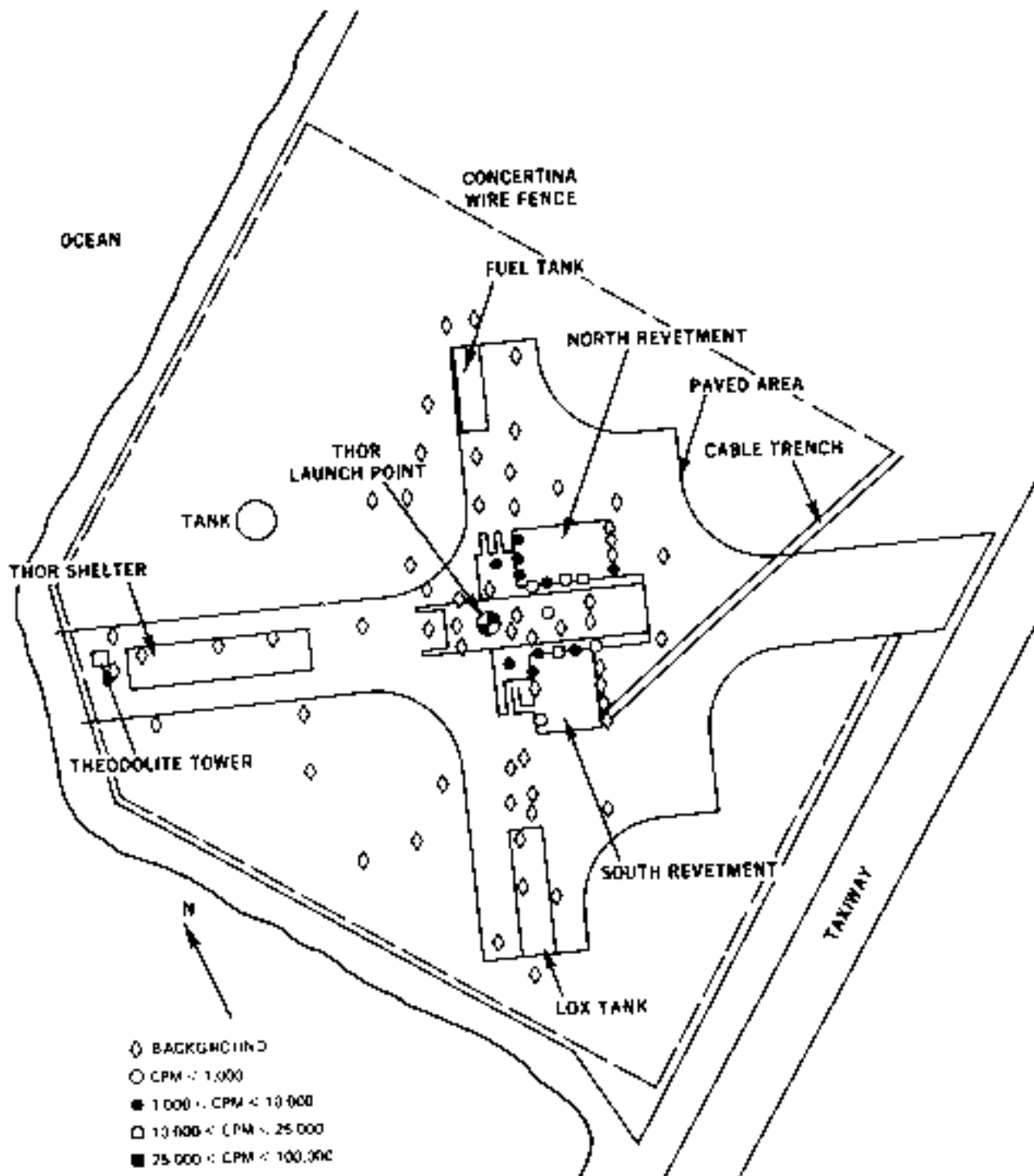
Figure 102. Thor launch pad contamination levels, 23 November 1962 after ODMINIC (source: Reference C.2052).
