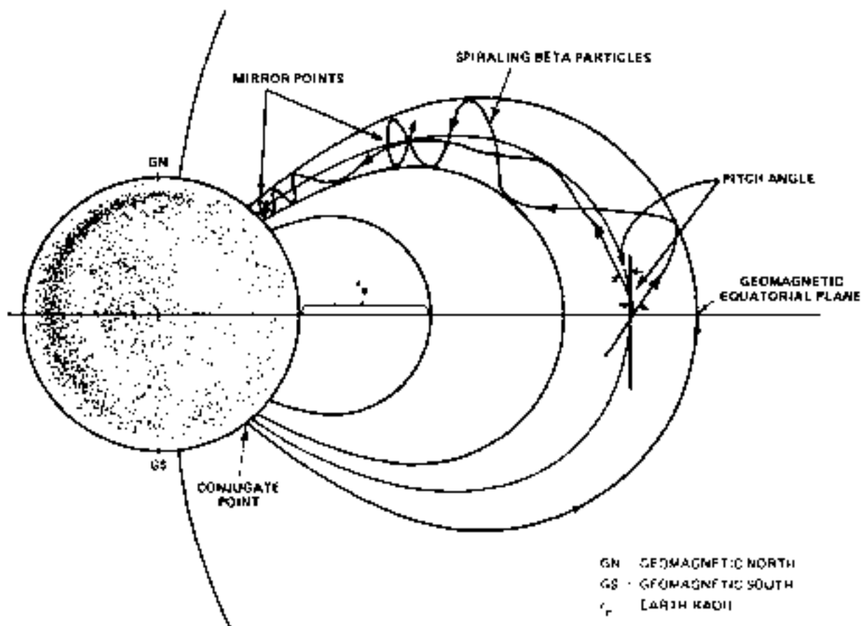
Figure 86. Earth's magnetic field.
