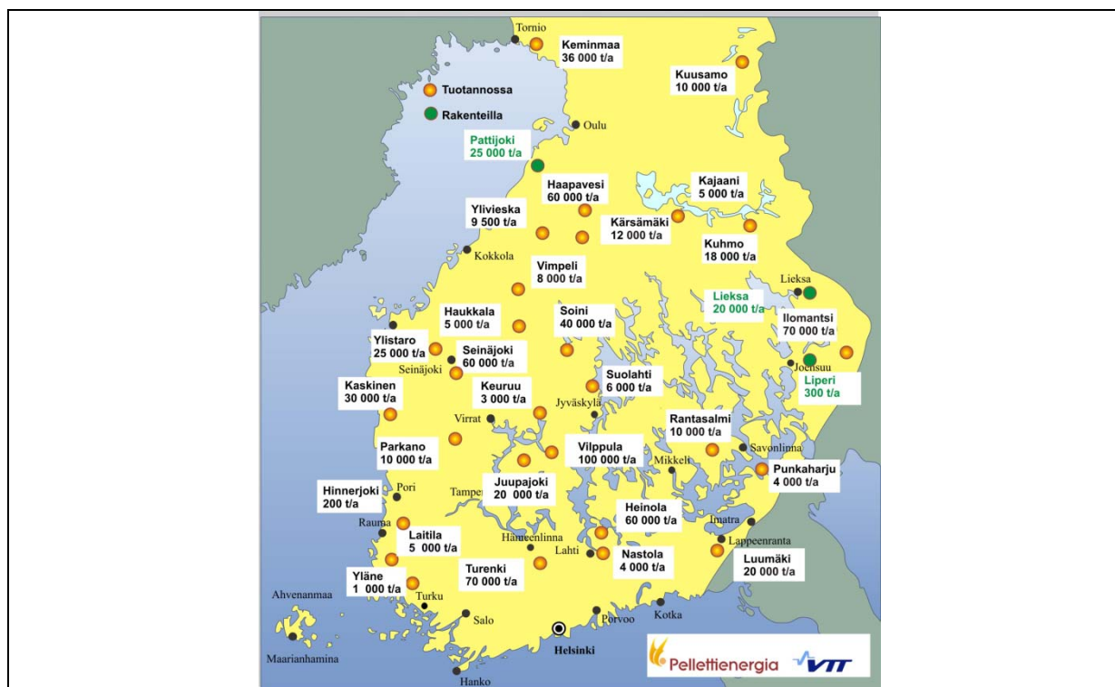
Figure 2.18. The locations and production capacities of Finnish wood pellet mills at the beginning of 2011. (brown spot = existing mill, green spot = under construction). Figure from Pellettienergiayhdistys ry.
