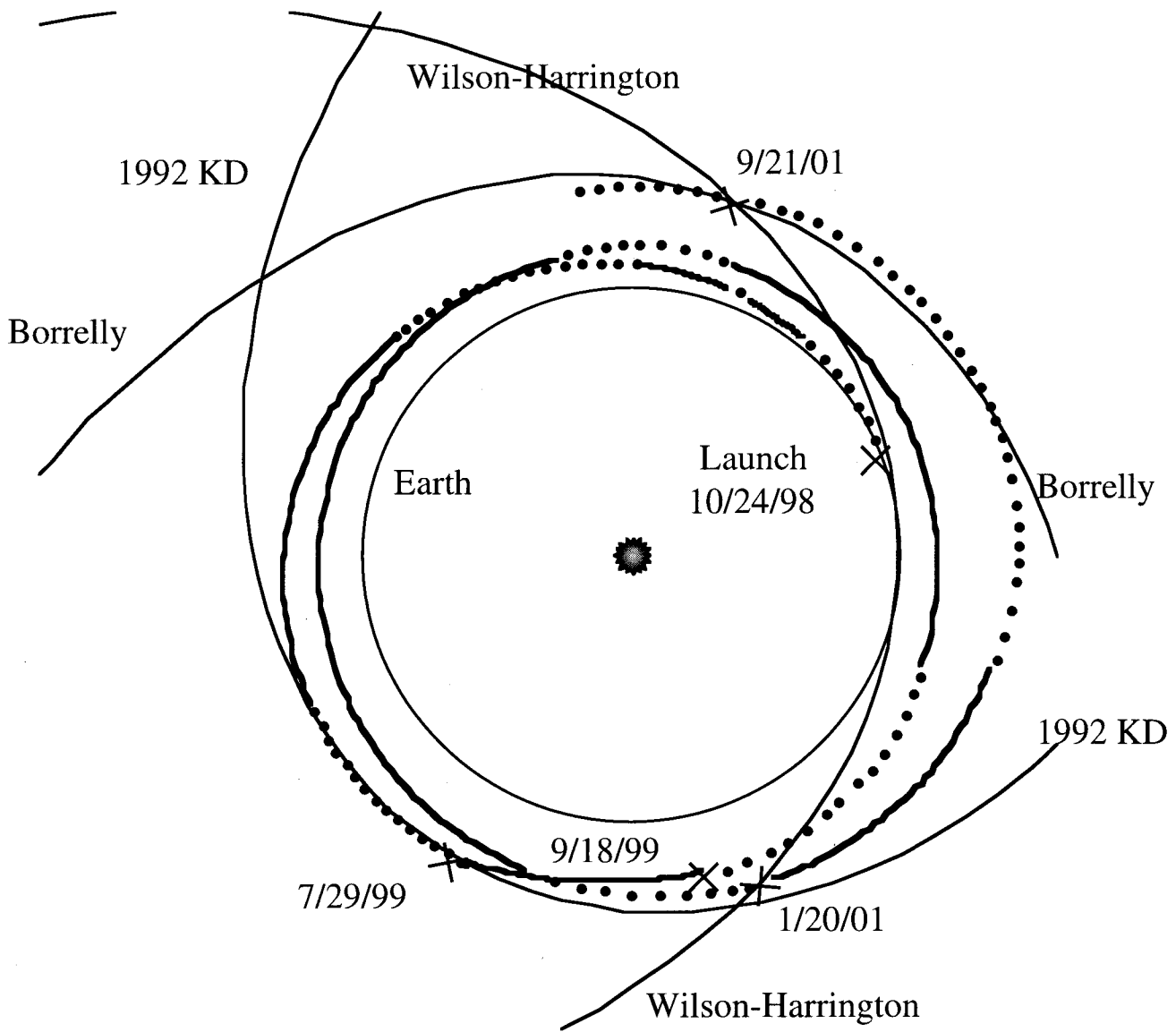
Figure 1. DS1 trajectory for the primary mission (through September 18, 1999) and proposed extended mission. The dotted portion indicates the IPS thrust is on; the solid portion is for ballistic coast.
