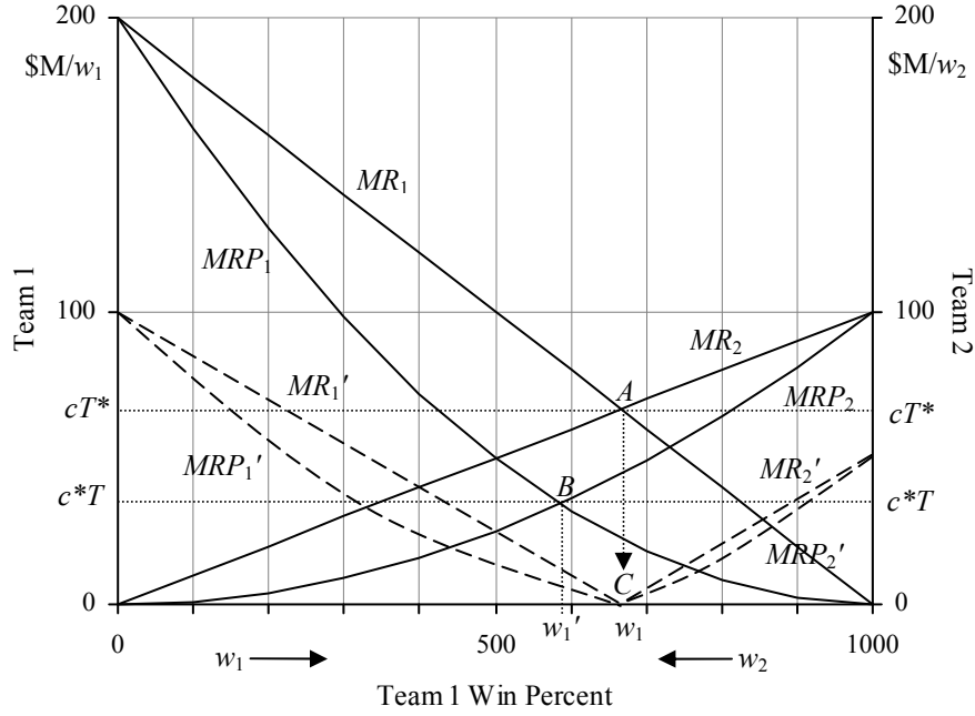
Fig. 1 Invariance Proposition
