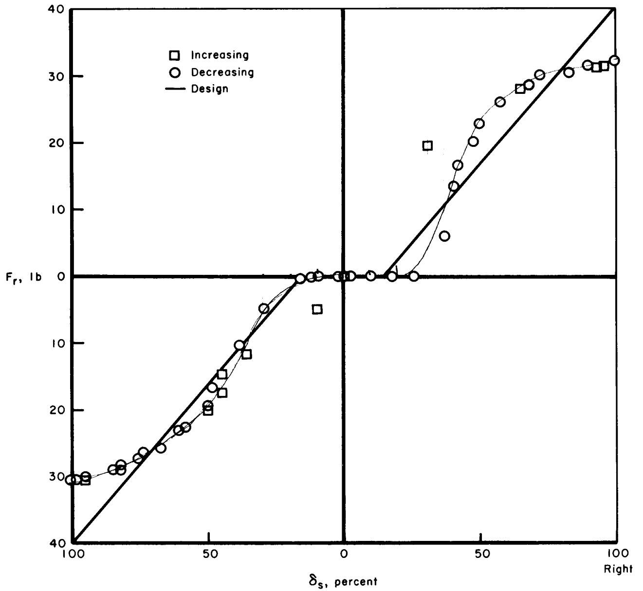
(b) Roll axis; maximum \delta_s = \pm 18^\circ .
