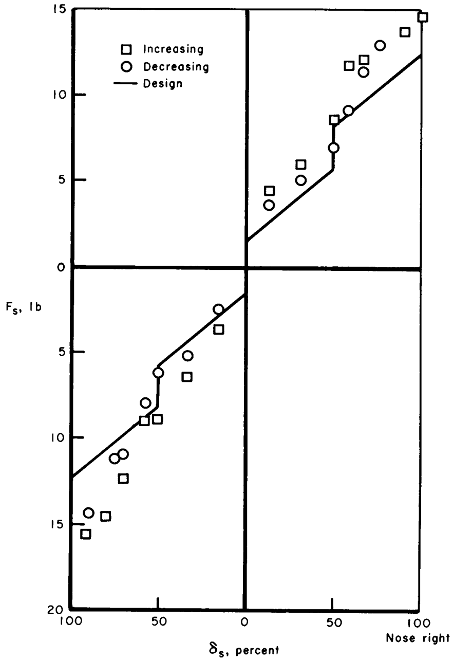
(c) Yaw axis; maximum \delta_s = \pm 8^\circ 2' .
