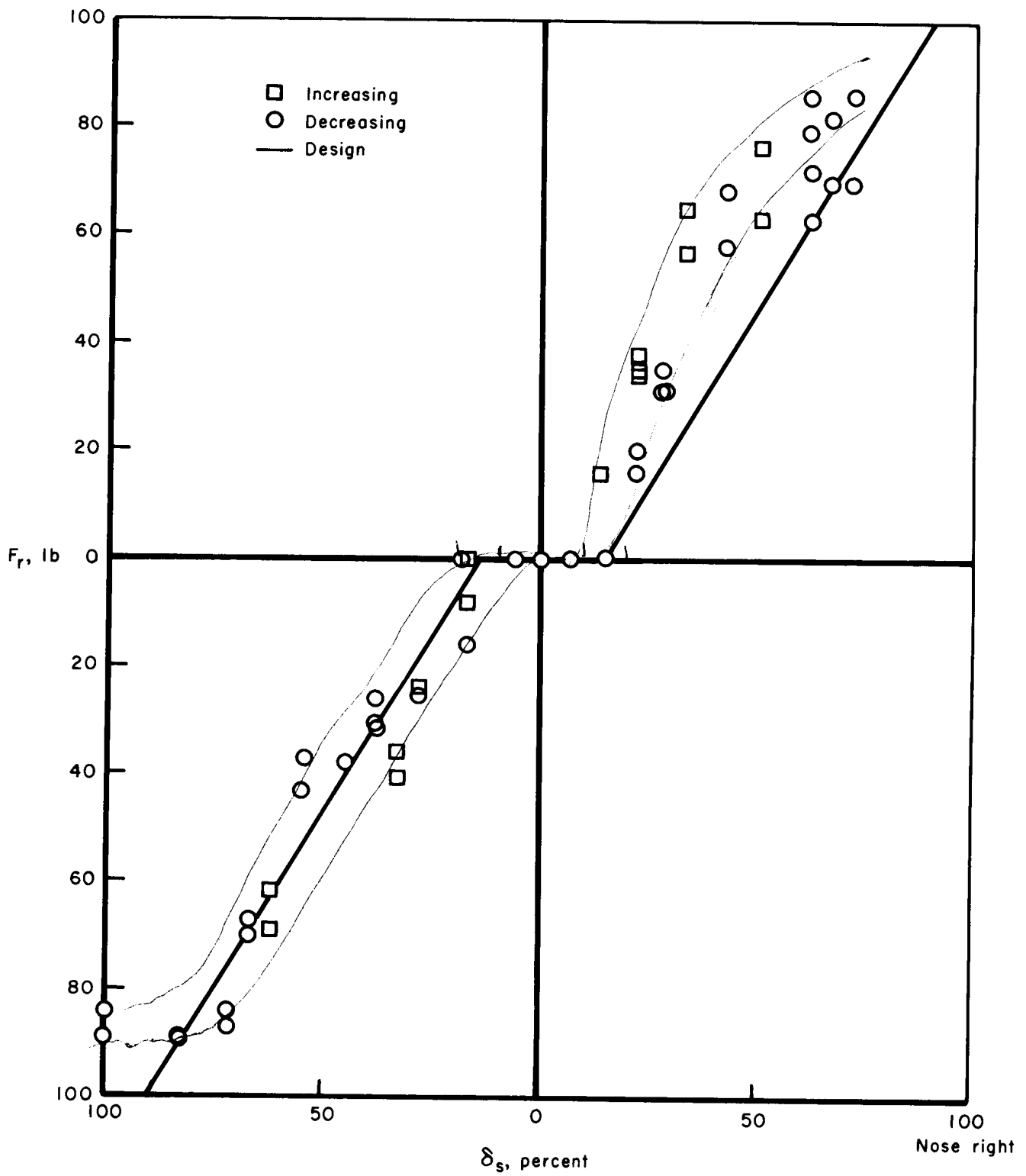
(c) Yaw axis; maximum \delta_S = \pm 8^\circ 2' .
