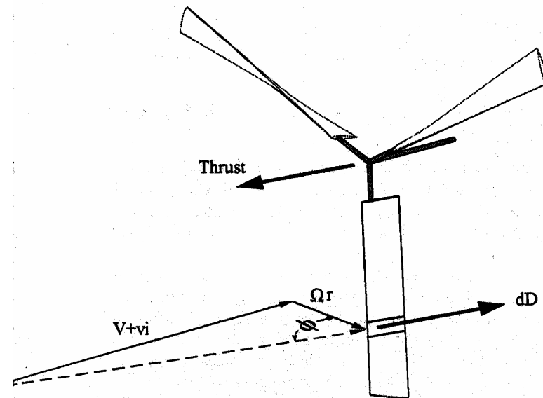
Figure D. Sketch of Prop-rotor
