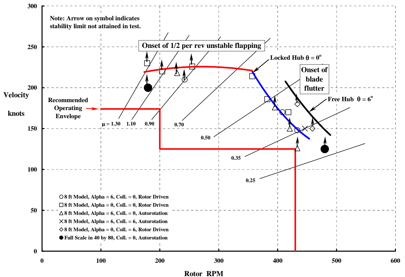
Figure 13. The XV-1 Recommended Operating Envelope Developed From Model and Full Scale Wind Tunnel Tests.
