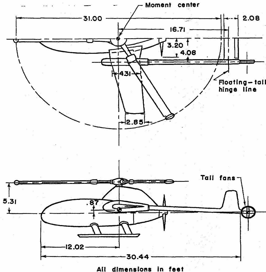
Figure 2.- General arrangement of the XV-1 convertiplane.
