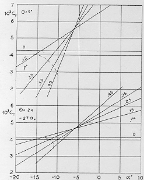
FIG. 7. Comparison between fixed-pitch rotor ( above ) and rotor with pitch-cone change ( below ). Thrust coefficient c_T against \alpha with advance ratio \mu as parameter. Dashed lines for constant c_Q/c_T equal to c_Q/c_T in hovering.
