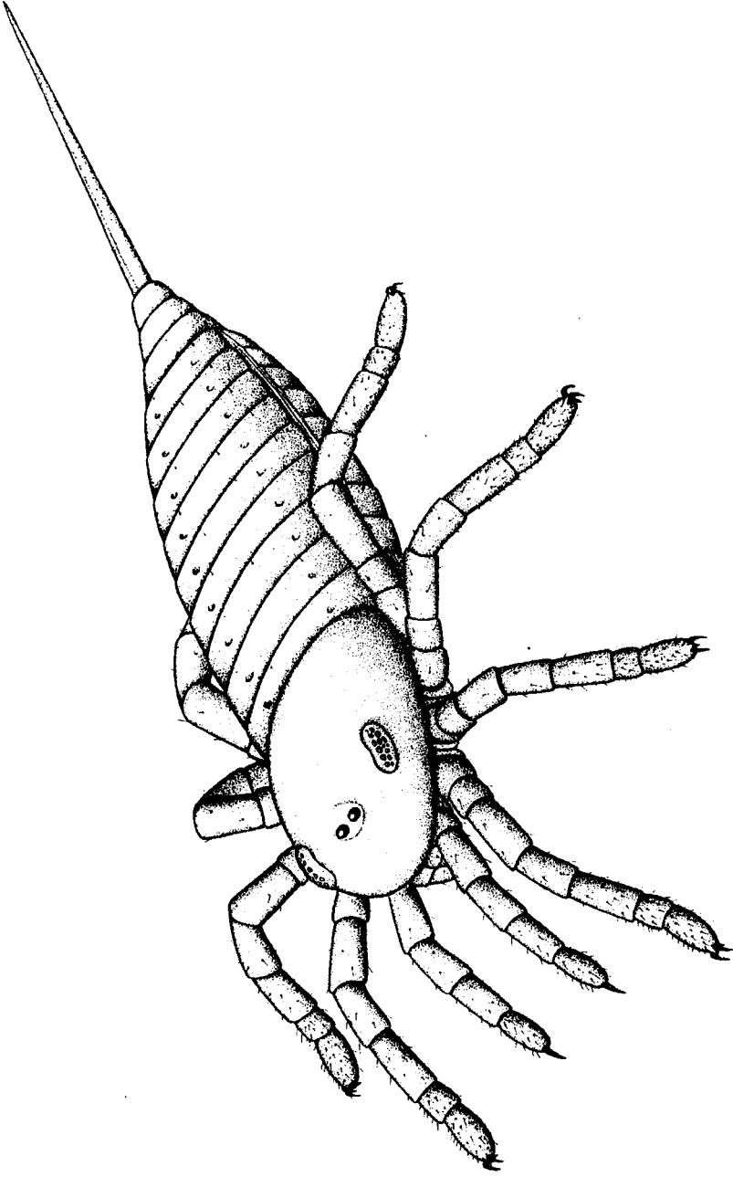
Fig. 2. Reconstruction of a hypothetical common ancestor of the (nonscorpion?) arachnids. The model shows the plesiomorphic character states of a twelve-segmented opisthosoma, an undivided telson, double femora and multifaceted lateral eyes. See text for details.
