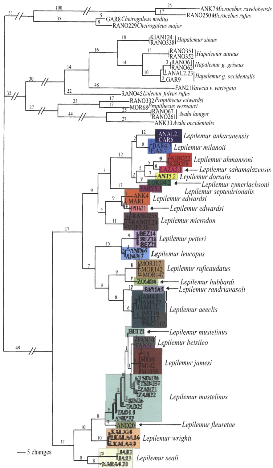
Figure 4. Phylogeny derived from combined 12S rDNA fragment sequence data from 54 haplotypes from 211 Lepilemur individuals (one of 128 most parsimonious trees). Values above branches indicate number of changes between nodes. Length = 1,080; CI = 0.5139; RI = 0.8629; RC = 0.4434; HI = 0.5132.
