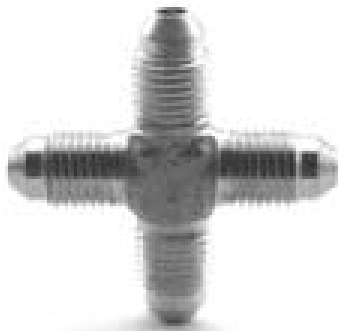
CROSS, Tube
