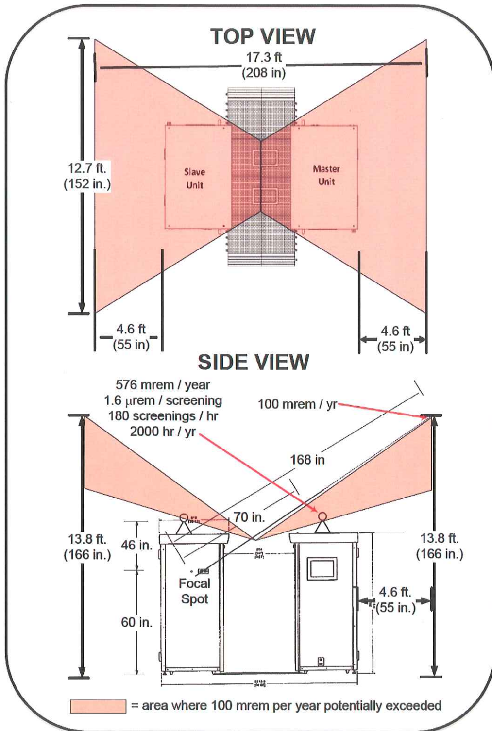
Figure 8-11. Dose to General Public Above Units
