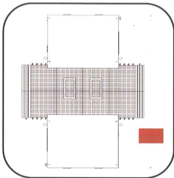
Figure 5-2. Top View of the Secure 1000 in Single Pose Configuration (Reference [4])
