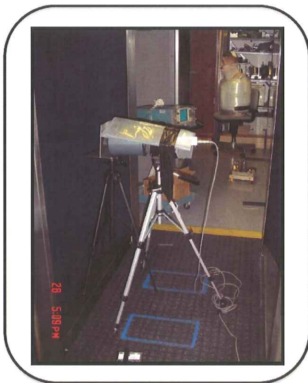
Figure 8-3. Ion Chamber Configuration for HVL Readings
