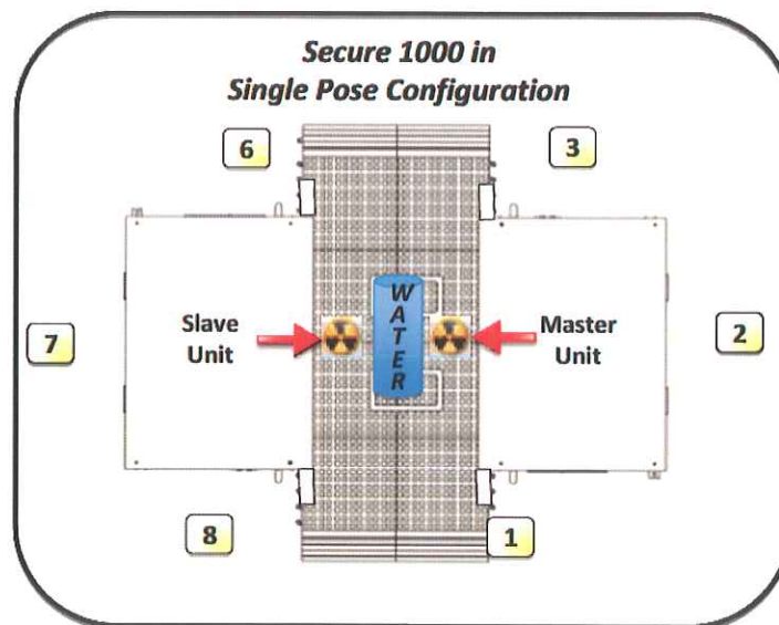
Figure 8-15. Locations for Leakage Dose Measurements
