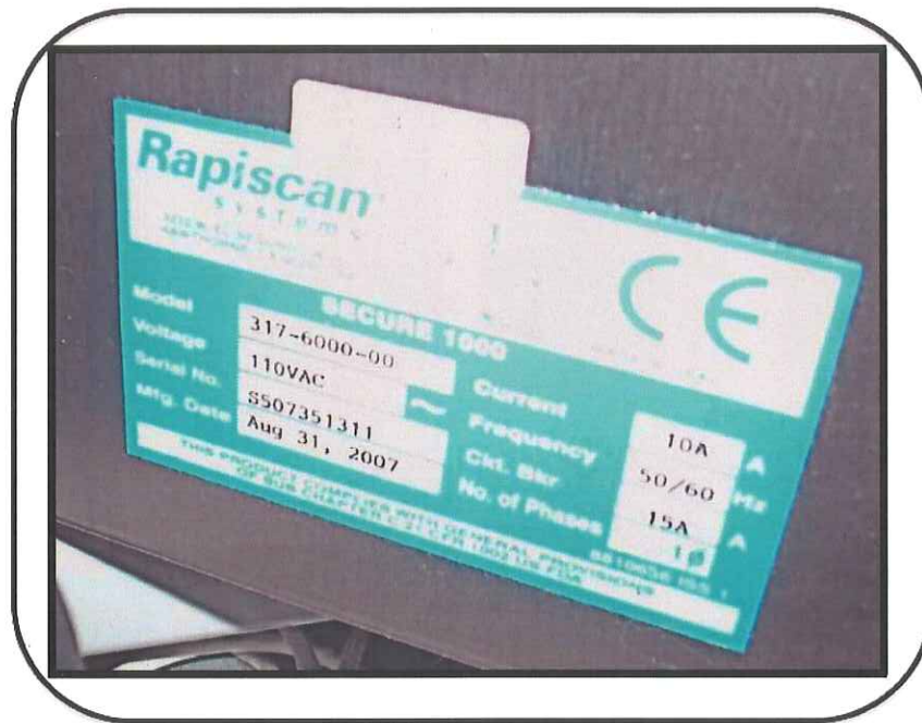
Figure 8-24: Secure 1000 in Single Pose Configuration Label
